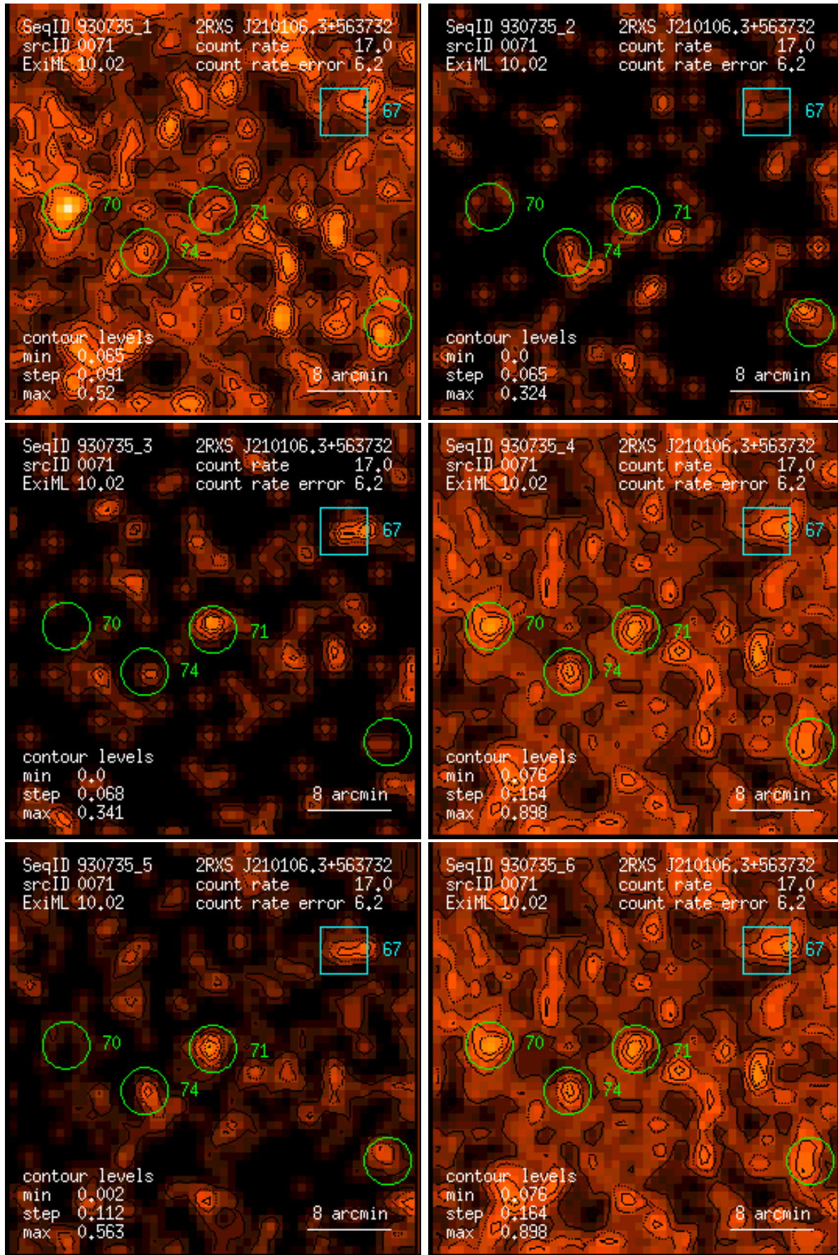
Figure 71: RASS 930735: detection 0071: band rate images, Gaussian filter: (1) PSPC channels 11 – 41, (2) 52 – 90, (3) 91 – 201, (4) 11 – 235, (5) 52 – 201, (6) 11 – 201. Broad band rates in counts/ks. Band rate contour levels in counts/ks/arcmin 2 .
