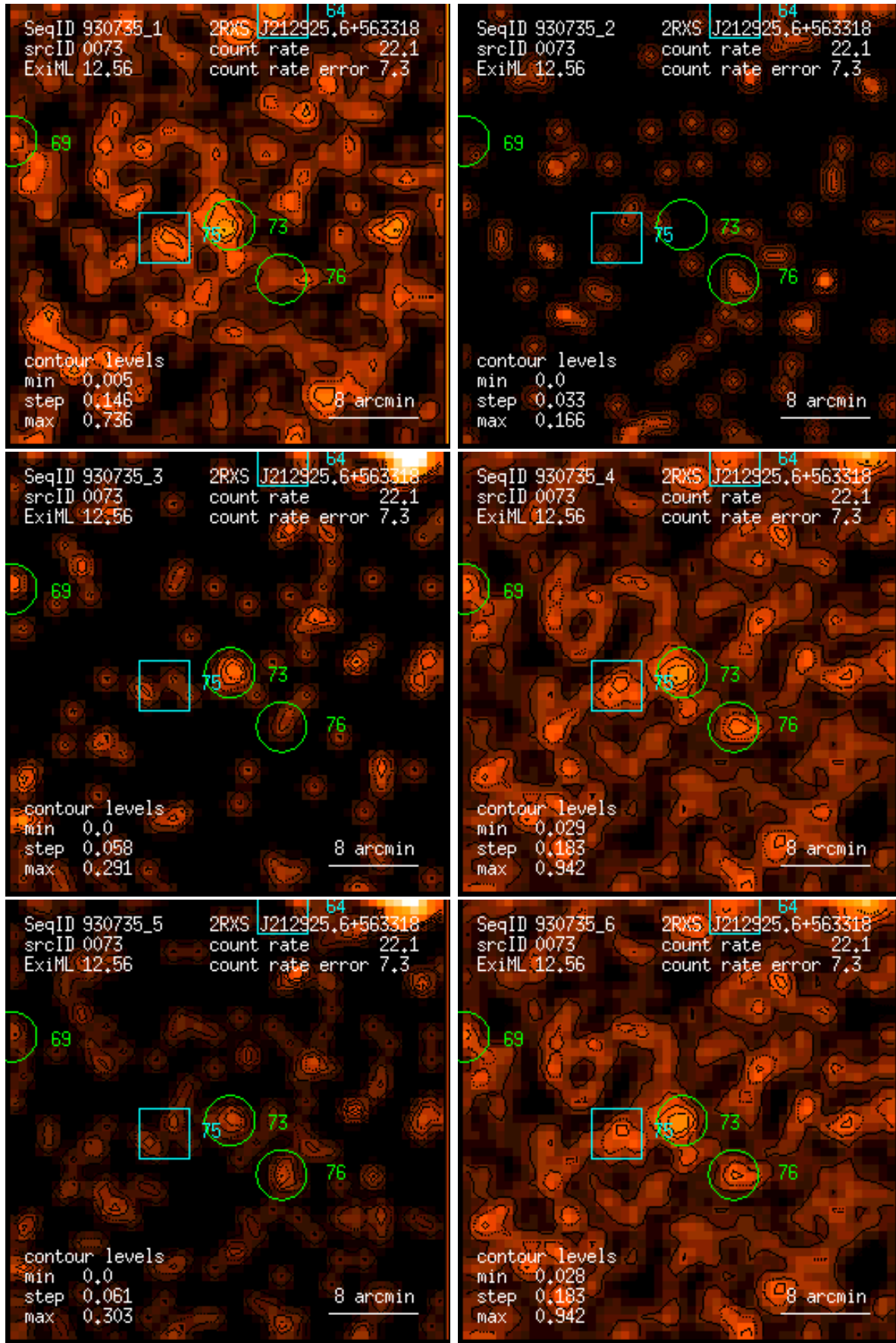
Figure 73: RASS 930735: detection 0073: band rate images, Gaussian filter: (1) PSPC channels 11 – 41, (2) 52 – 90, (3) 91 – 201, (4) 11 – 235, (5) 52 – 201, (6) 11 – 201. Broad band rates in counts/ks. Band rate contour levels in counts/ks/arcmin 2 .
