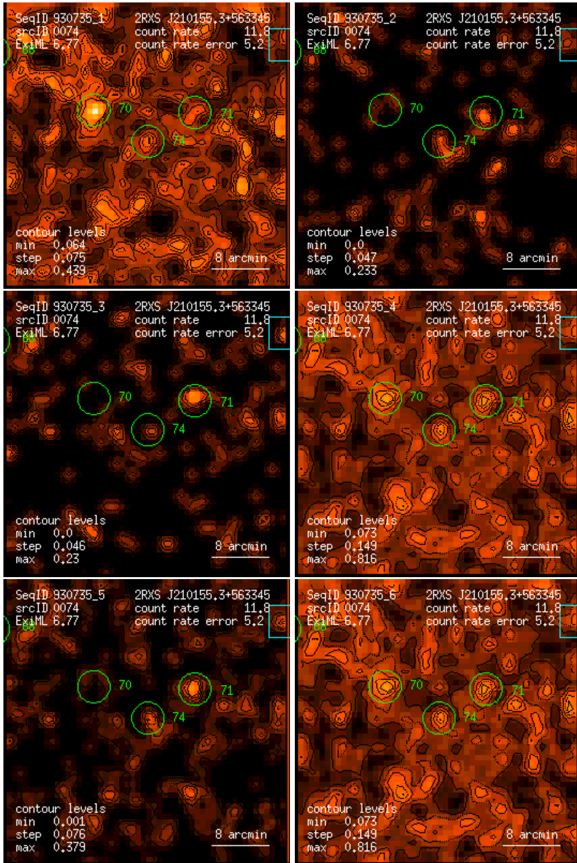
Figure 74: RASS 930735: detection 0074: band rate images, Gaussian filter: (1) PSPC channels 11 – 41, (2) 52 – 90, (3) 91 – 201, (4) 11 – 235, (5) 52 – 201, (6) 11 – 201. Broad band rates in counts/ks. Band rate contour levels in counts/ks/arcmin 2 .
