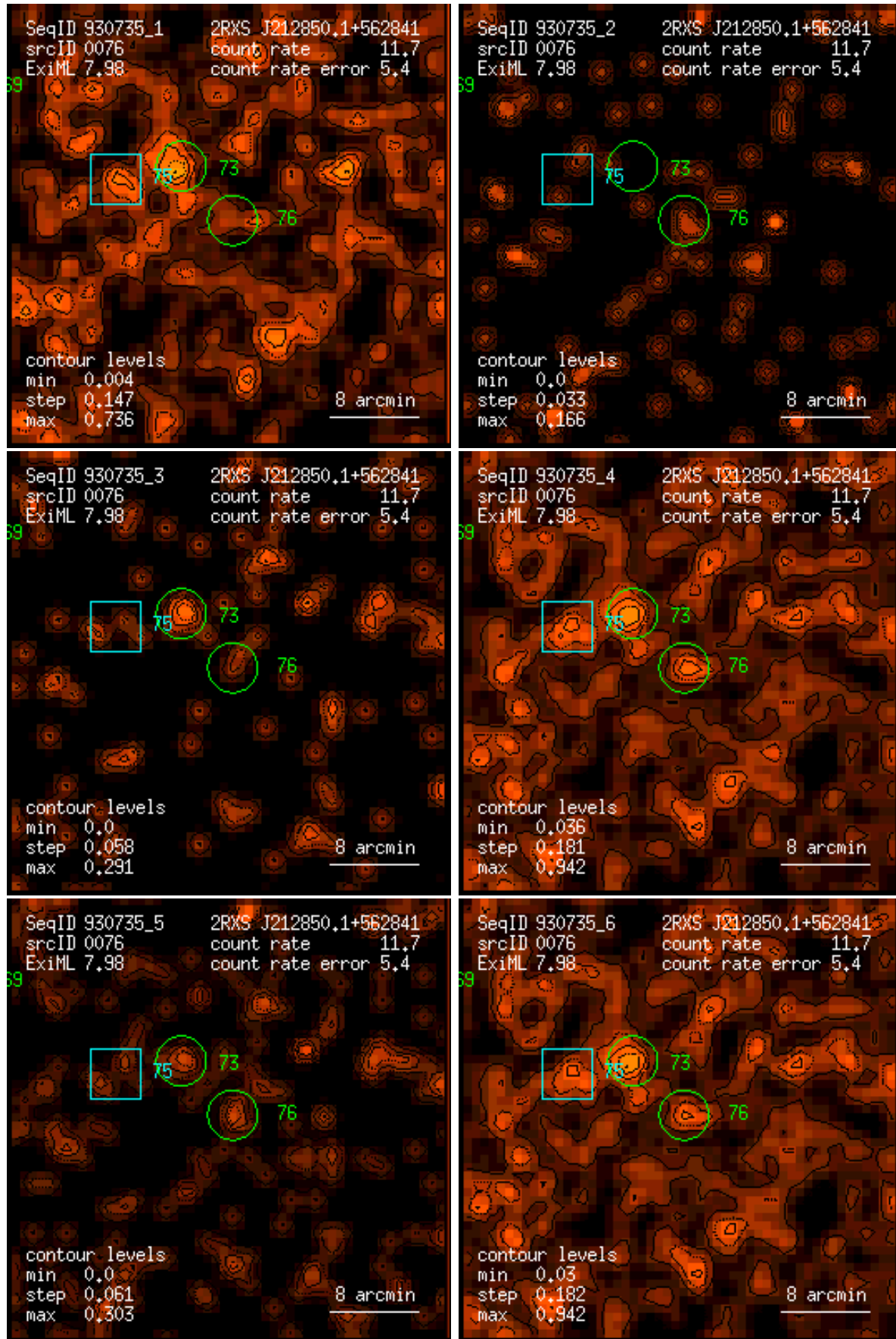
Figure 76: RASS 930735: detection 0076: band rate images, Gaussian filter: (1) PSPC channels 11 – 41, (2) 52 – 90, (3) 91 – 201, (4) 11 – 235, (5) 52 – 201, (6) 11 – 201. Broad band rates in counts/ks. Band rate contour levels in counts/ks/arcmin 2 .
