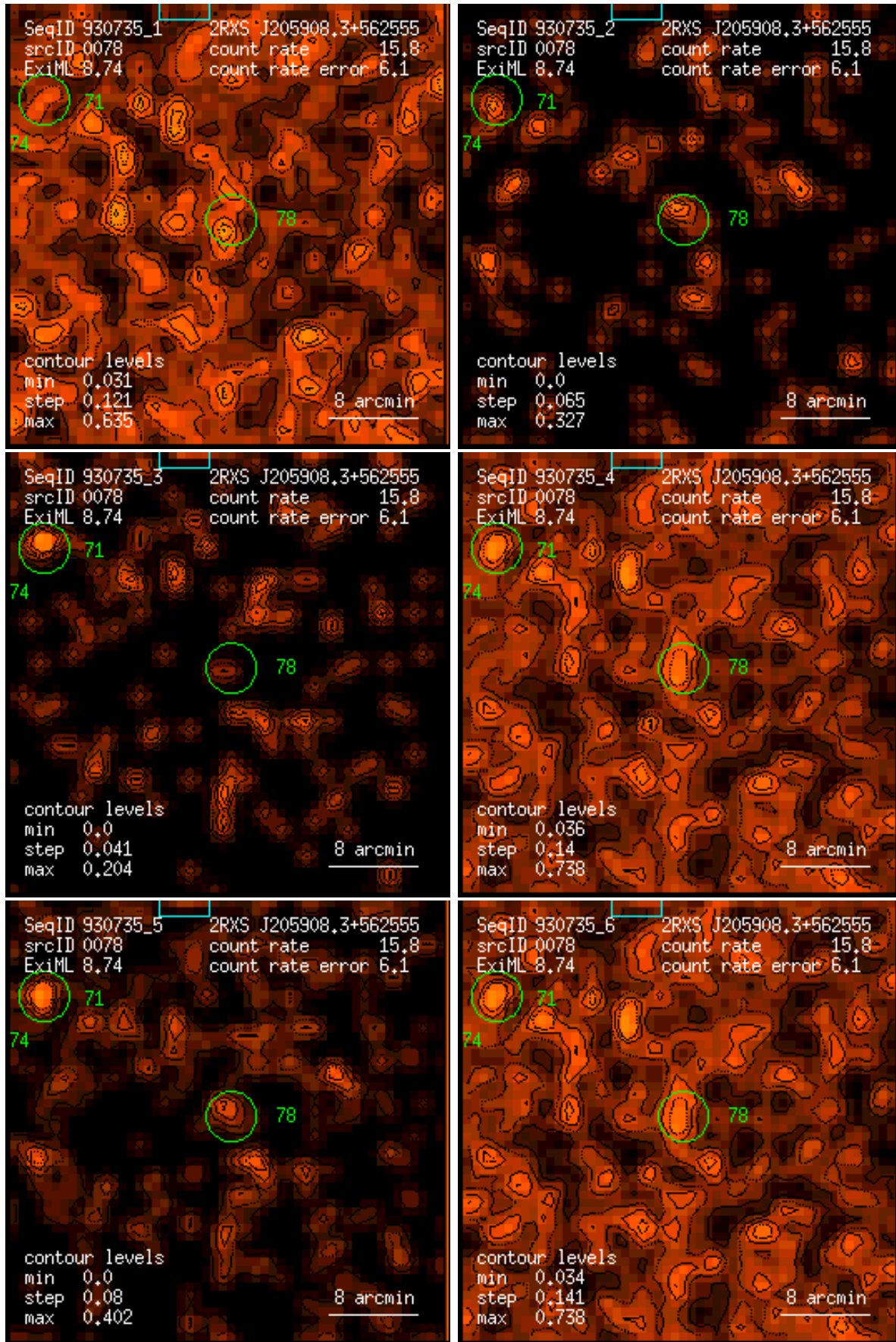
Figure 78: RASS 930735: detection 0078: band rate images, Gaussian filter: (1) PSPC channels 11 – 41, (2) 52 – 90, (3) 91 – 201, (4) 11 – 235, (5) 52 – 201, (6) 11 – 201. Broad band rates in counts/ks. Band rate contour levels in counts/ks/arcmin 2 .
