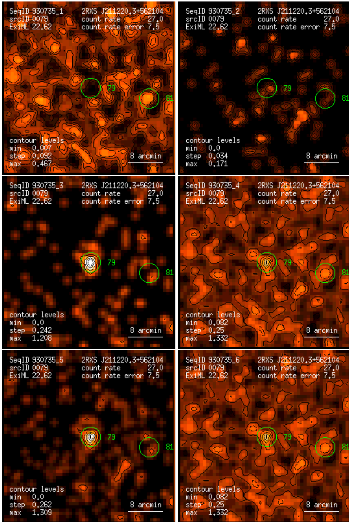
Figure 79: RASS 930735: detection 0079: band rate images, Gaussian filter: (1) PSPC channels 11 – 41, (2) 52 – 90, (3) 91 – 201, (4) 11 – 235, (5) 52 – 201, (6) 11 – 201. Broad band rates in counts/ks. Band rate contour levels in counts/ks/arcmin 2 .
