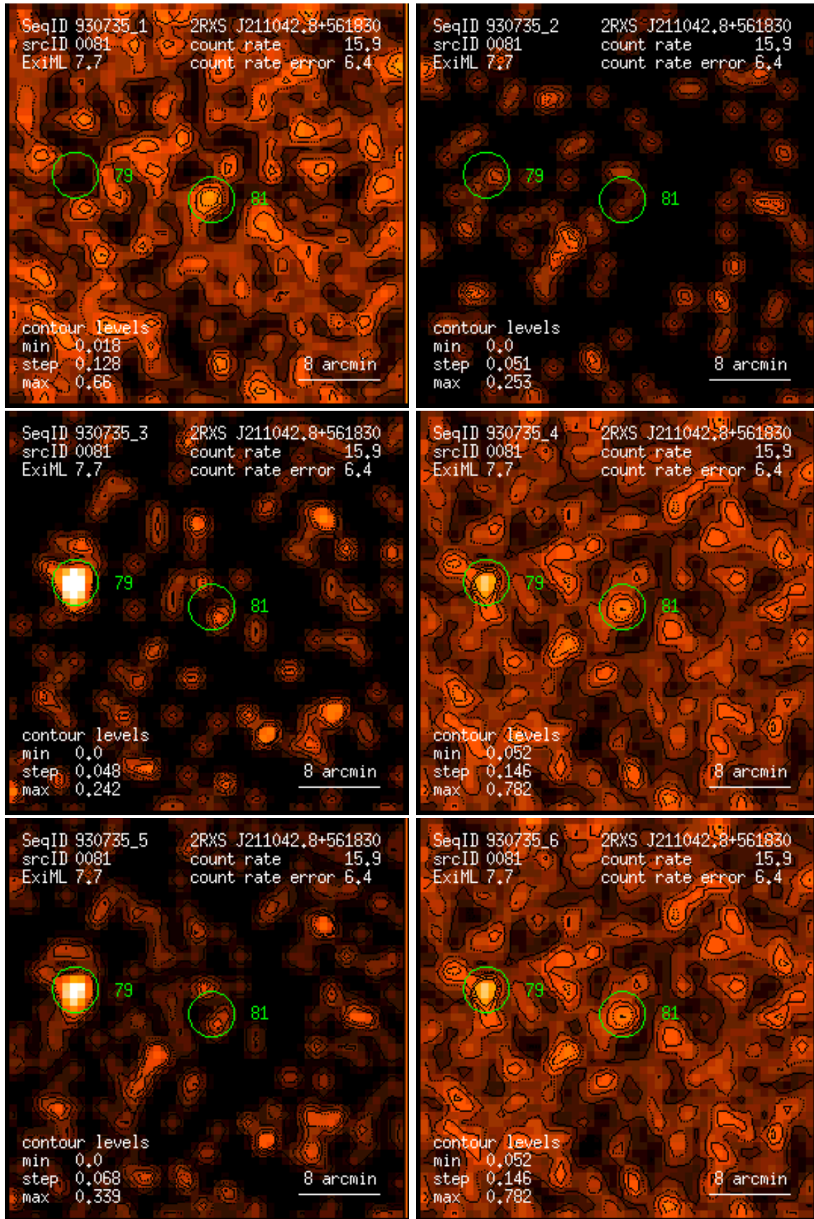
Figure 81: RASS 930735: detection 0081: band rate images, Gaussian filter: (1) PSPC channels 11 – 41, (2) 52 – 90, (3) 91 – 201, (4) 11 – 235, (5) 52 – 201, (6) 11 – 201. Broad band rates in counts/ks. Band rate contour levels in counts/ks/arcmin 2 .
