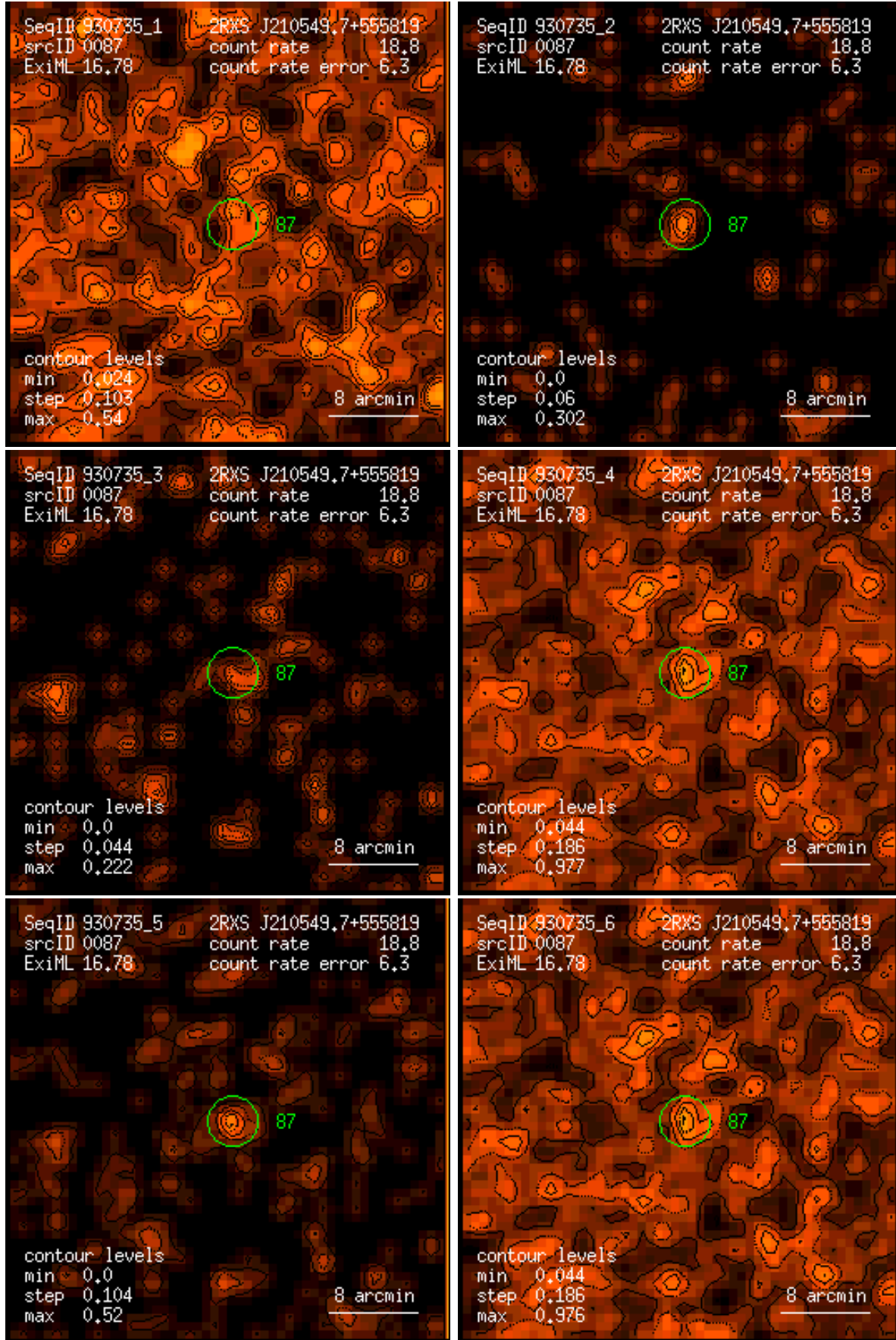
Figure 87: RASS 930735: detection 0087: band rate images, Gaussian filter: (1) PSPC channels 11 – 41, (2) 52 – 90, (3) 91 – 201, (4) 11 – 235, (5) 52 – 201, (6) 11 – 201. Broad band rates in counts/ks. Band rate contour levels in counts/ks/arcmin 2 .
