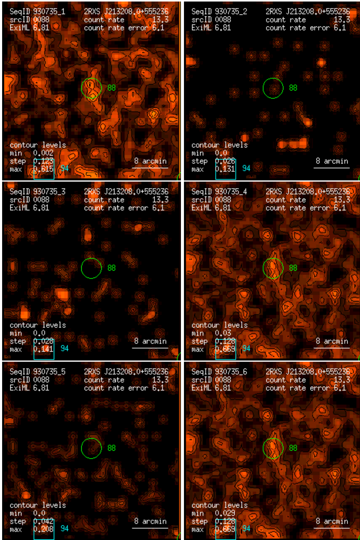
Figure 88: RASS 930735: detection 0088: band rate images, Gaussian filter: (1) PSPC channels 11 – 41, (2) 52 – 90, (3) 91 – 201, (4) 11 – 235, (5) 52 – 201, (6) 11 – 201. Broad band rates in counts/ks. Band rate contour levels in counts/ks/arcmin 2 .
