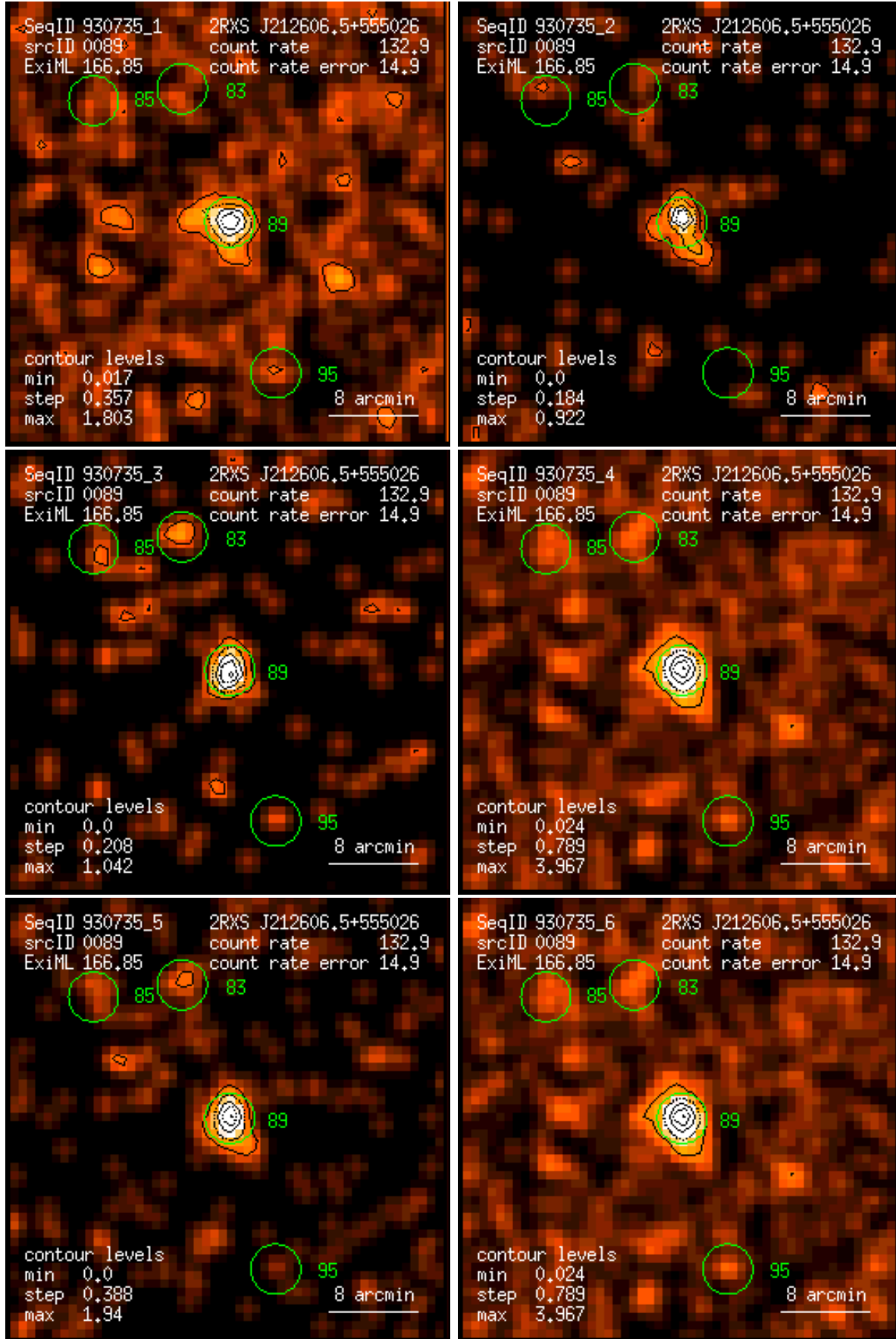
Figure 89: RASS 930735: detection 0089: band rate images, Gaussian filter: (1) PSPC channels 11 – 41, (2) 52 – 90, (3) 91 – 201, (4) 11 – 235, (5) 52 – 201, (6) 11 – 201. Broad band rates in counts/ks. Band rate contour levels in counts/ks/arcmin 2 .
