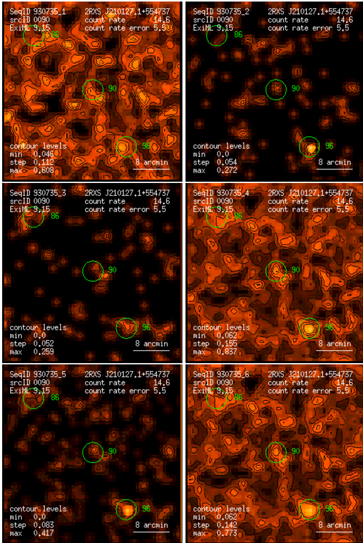
Figure 90: RASS 930735: detection 0090: band rate images, Gaussian filter: (1) PSPC channels 11 – 41, (2) 52 – 90, (3) 91 – 201, (4) 11 – 235, (5) 52 – 201, (6) 11 – 201. Broad band rates in counts/ks. Band rate contour levels in counts/ks/arcmin 2 .
