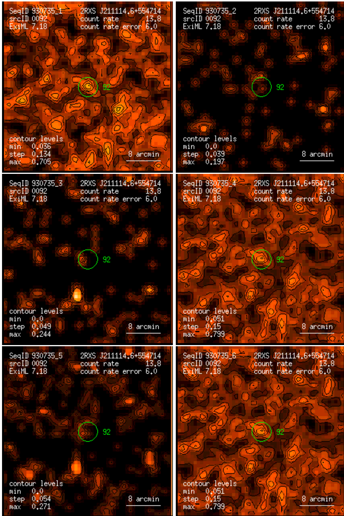
Figure 92: RASS 930735: detection 0092: band rate images, Gaussian filter: (1) PSPC channels 11 – 41, (2) 52 – 90, (3) 91 – 201, (4) 11 – 235, (5) 52 – 201, (6) 11 – 201. Broad band rates in counts/ks. Band rate contour levels in counts/ks/arcmin 2 .
