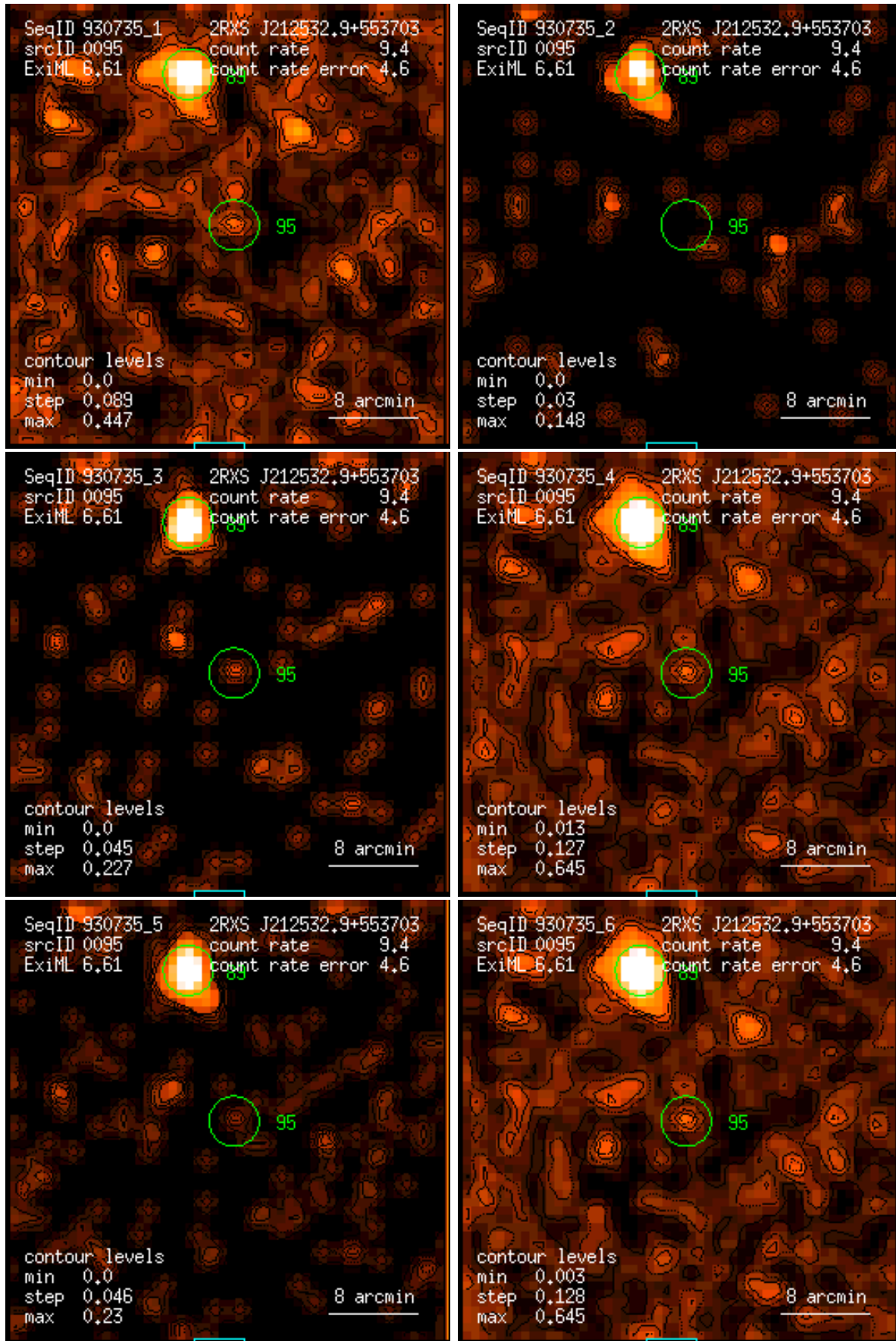
Figure 95: RASS 930735: detection 0095: band rate images, Gaussian filter: (1) PSPC channels 11 – 41, (2) 52 – 90, (3) 91 – 201, (4) 11 – 235, (5) 52 – 201, (6) 11 – 201. Broad band rates in counts/ks. Band rate contour levels in counts/ks/arcmin 2 .
