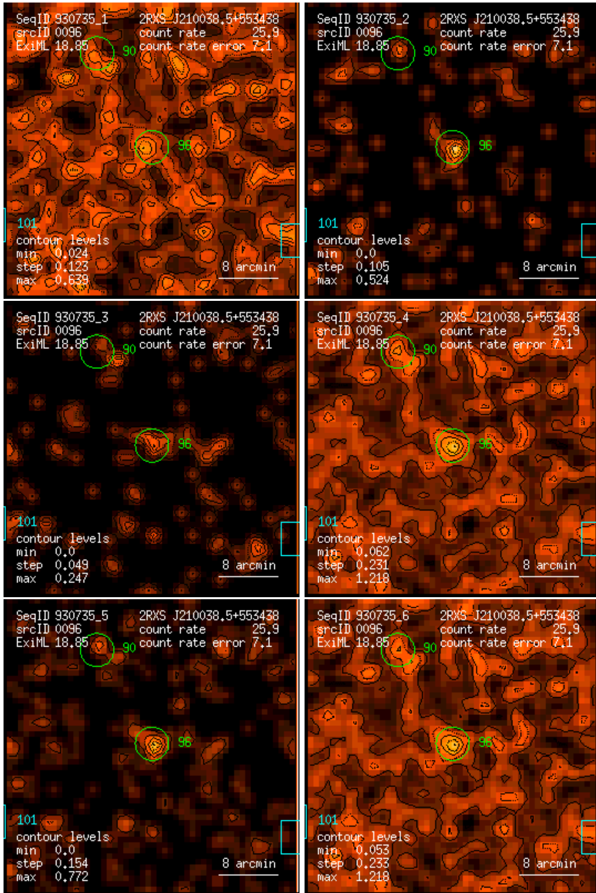
Figure 96: RASS 930735: detection 0096: band rate images, Gaussian filter: (1) PSPC channels 11 – 41, (2) 52 – 90, (3) 91 – 201, (4) 11 – 235, (5) 52 – 201, (6) 11 – 201. Broad band rates in counts/ks. Band rate contour levels in counts/ks/arcmin 2 .
