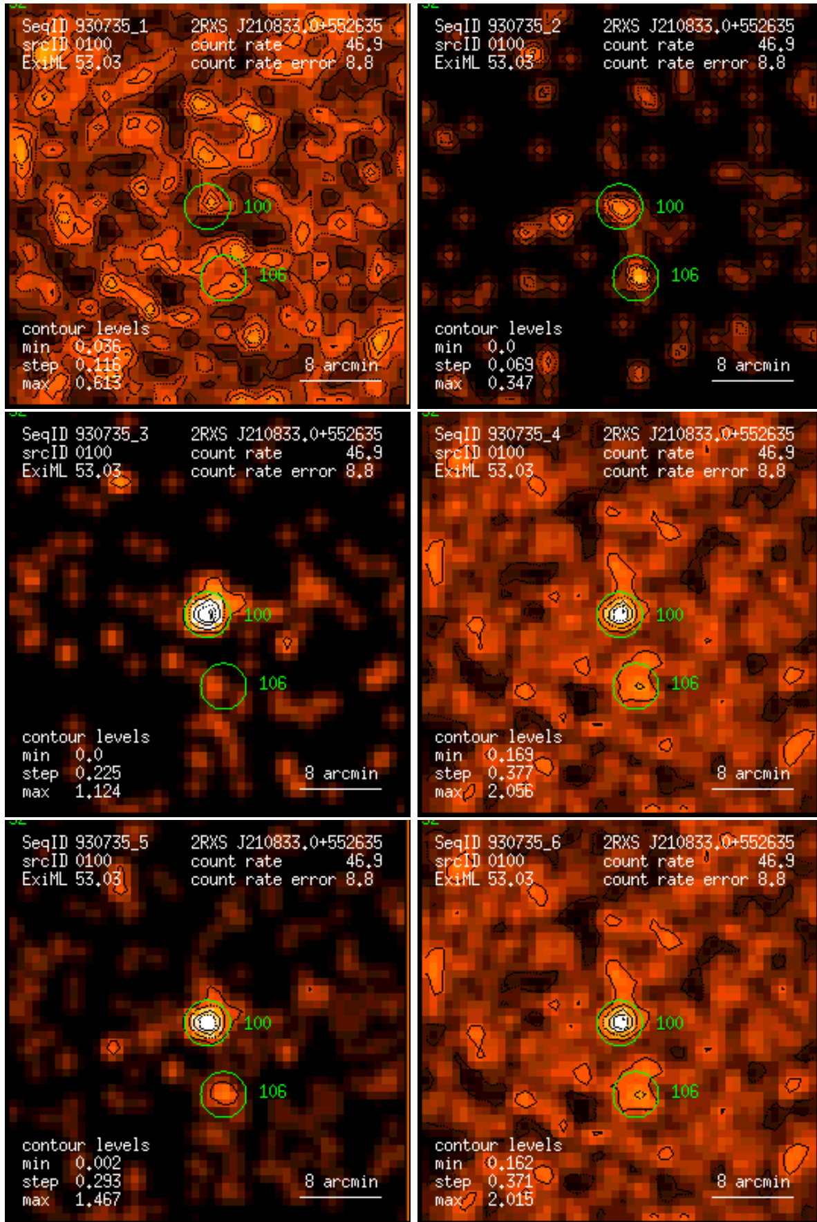
Figure 100: RASS 930735: detection 0100: band rate images, Gaussian filter: (1) PSPC channels 11 – 41, (2) 52 – 90, (3) 91 – 201, (4) 11 – 235, (5) 52 – 201, (6) 11 – 201. Broad band rates in counts/ks. Band rate contour levels in counts/ks/arcmin 2 .
