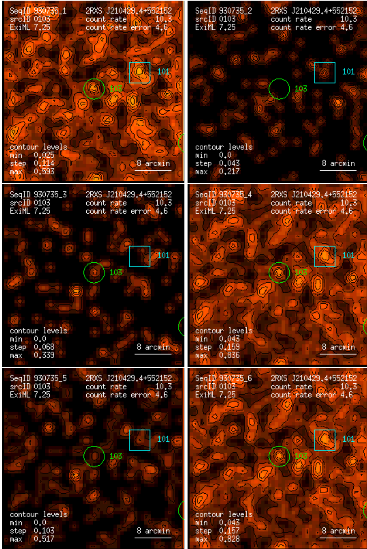
Figure 103: RASS 930735: detection 0103: band rate images, Gaussian filter: (1) PSPC channels 11 – 41, (2) 52 – 90, (3) 91 – 201, (4) 11 – 235, (5) 52 – 201, (6) 11 – 201. Broad band rates in counts/ks. Band rate contour levels in counts/ks/arcmin 2 .
