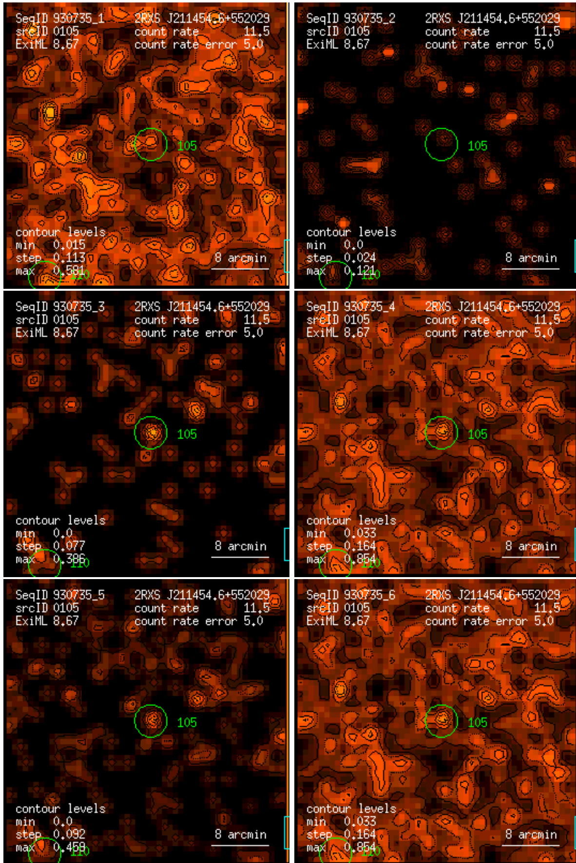
Figure 105: RASS 930735: detection 0105: band rate images, Gaussian filter: (1) PSPC channels 11 – 41, (2) 52 – 90, (3) 91 – 201, (4) 11 – 235, (5) 52 – 201, (6) 11 – 201. Broad band rates in counts/ks. Band rate contour levels in counts/ks/arcmin 2 .
