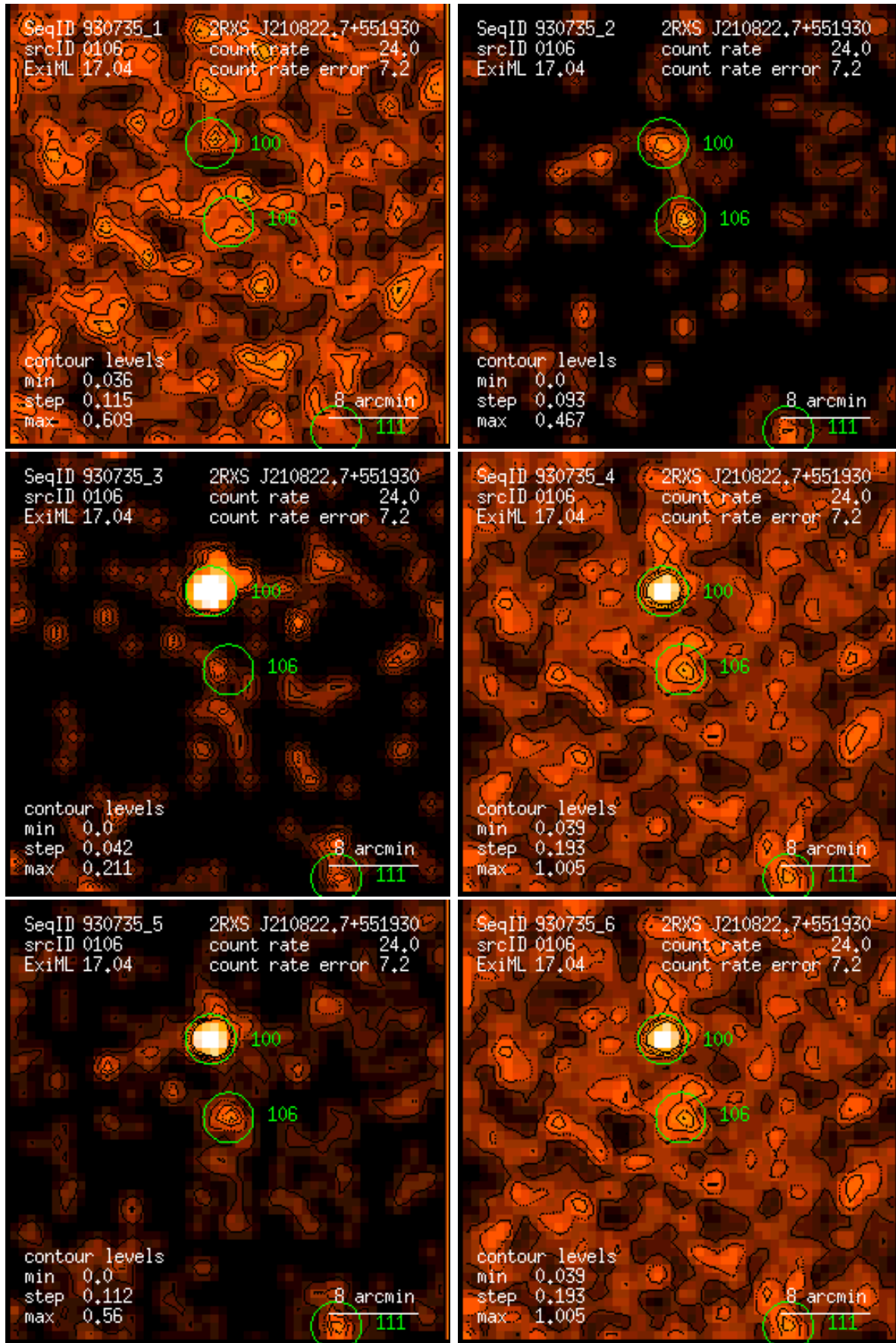
Figure 106: RASS 930735: detection 0106: band rate images, Gaussian filter: (1) PSPC channels 11 – 41, (2) 52 – 90, (3) 91 – 201, (4) 11 – 235, (5) 52 – 201, (6) 11 – 201. Broad band rates in counts/ks. Band rate contour levels in counts/ks/arcmin 2 .
