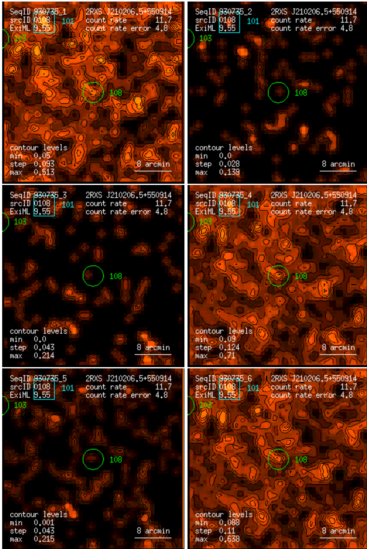
Figure 108: RASS 930735: detection 0108: band rate images, Gaussian filter: (1) PSPC channels 11 – 41, (2) 52 – 90, (3) 91 – 201, (4) 11 – 235, (5) 52 – 201, (6) 11 – 201. Broad band rates in counts/ks. Band rate contour levels in counts/ks/arcmin 2 .
