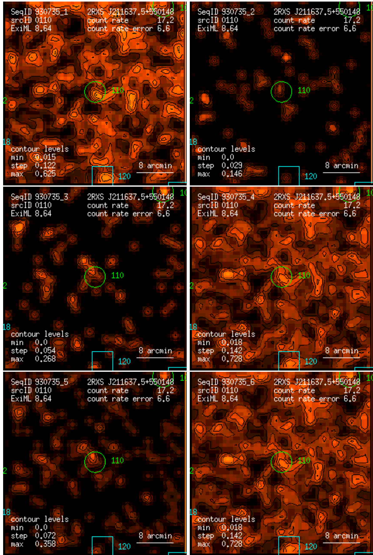
Figure 110: RASS 930735: detection 0110: band rate images, Gaussian filter: (1) PSPC channels 11 – 41, (2) 52 – 90, (3) 91 – 201, (4) 11 – 235, (5) 52 – 201, (6) 11 – 201. Broad band rates in counts/ks. Band rate contour levels in counts/ks/arcmin 2 .
