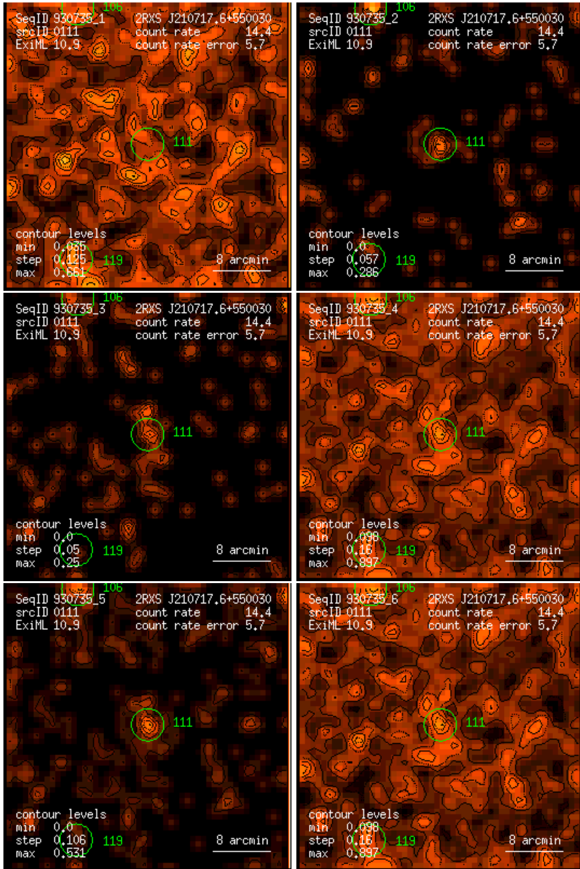
Figure 111: RASS 930735: detection 0111: band rate images, Gaussian filter: (1) PSPC channels 11 – 41, (2) 52 – 90, (3) 91 – 201, (4) 11 – 235, (5) 52 – 201, (6) 11 – 201. Broad band rates in counts/ks. Band rate contour levels in counts/ks/arcmin 2 .
