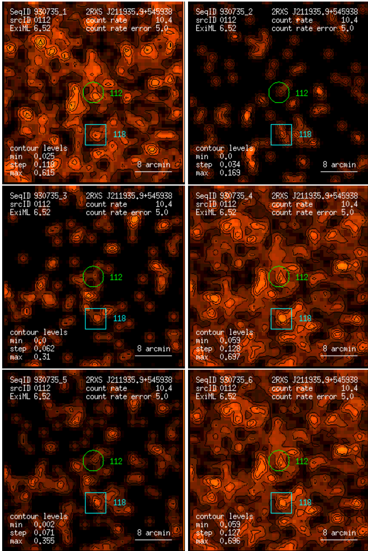
Figure 112: RASS 930735: detection 0112: band rate images, Gaussian filter: (1) PSPC channels 11 – 41, (2) 52 – 90, (3) 91 – 201, (4) 11 – 235, (5) 52 – 201, (6) 11 – 201. Broad band rates in counts/ks. Band rate contour levels in counts/ks/arcmin 2 .
