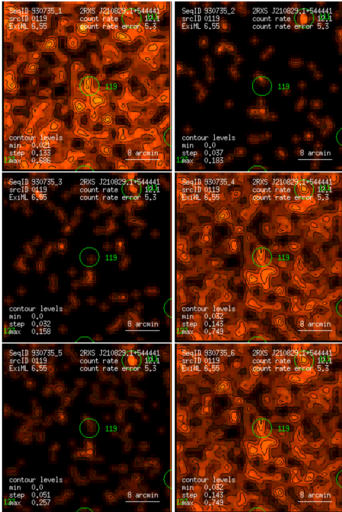
Figure 119: RASS 930735: detection 0119: band rate images, Gaussian filter: (1) PSPC channels 11 – 41, (2) 52 – 90, (3) 91 – 201, (4) 11 – 235, (5) 52 – 201, (6) 11 – 201. Broad band rates in counts/ks. Band rate contour levels in counts/ks/arcmin 2 .
