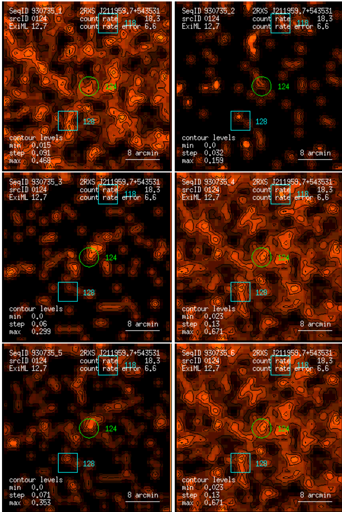
Figure 124: RASS 930735: detection 0124: band rate images, Gaussian filter: (1) PSPC channels 11 – 41, (2) 52 – 90, (3) 91 – 201, (4) 11 – 235, (5) 52 – 201, (6) 11 – 201. Broad band rates in counts/ks. Band rate contour levels in counts/ks/arcmin 2 .
