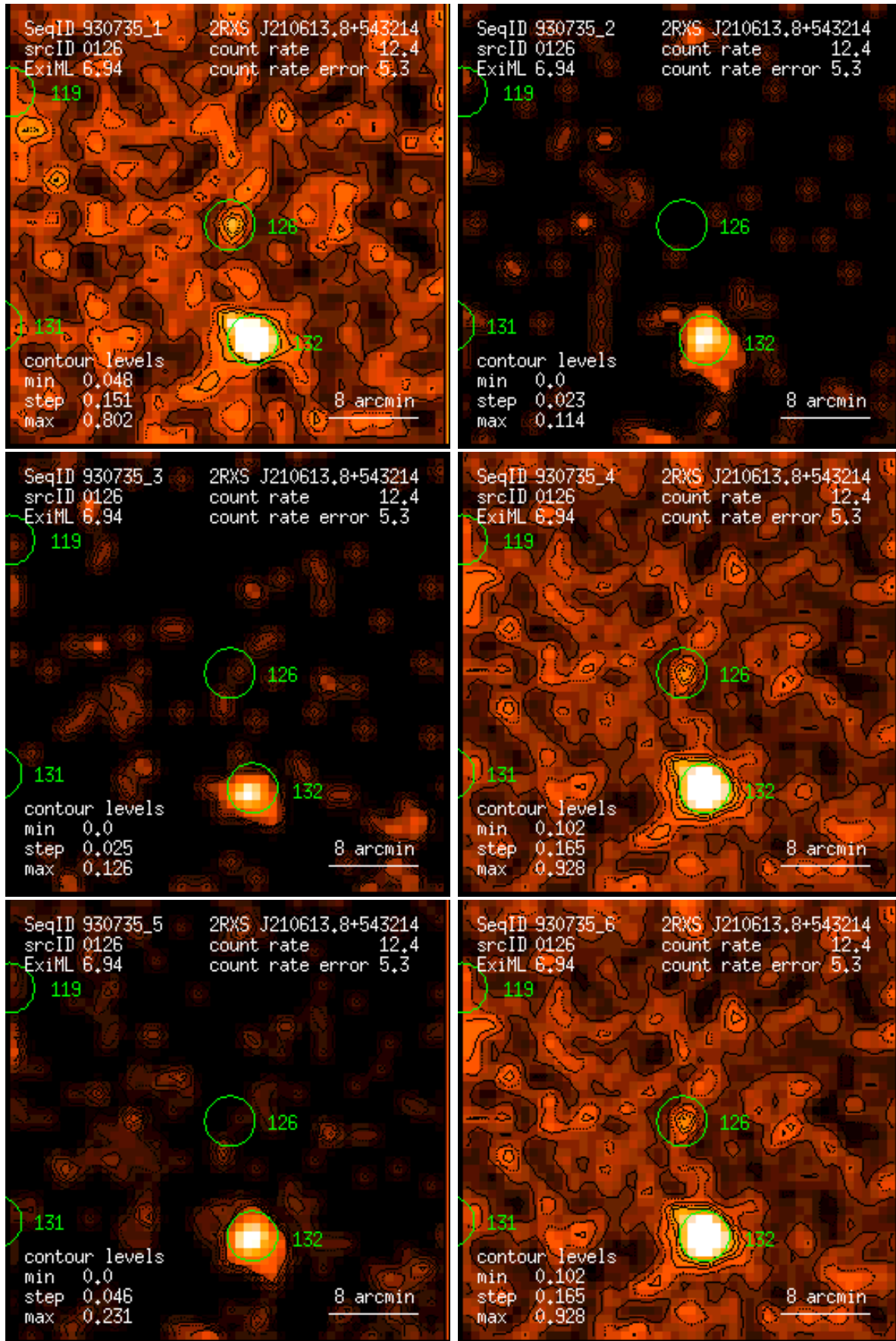
Figure 126: RASS 930735: detection 0126: band rate images, Gaussian filter: (1) PSPC channels 11 – 41, (2) 52 – 90, (3) 91 – 201, (4) 11 – 235, (5) 52 – 201, (6) 11 – 201. Broad band rates in counts/ks. Band rate contour levels in counts/ks/arcmin 2 .
