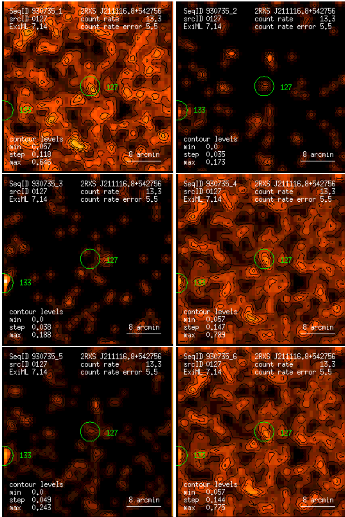
Figure 127: RASS 930735: detection 0127: band rate images, Gaussian filter: (1) PSPC channels 11 – 41, (2) 52 – 90, (3) 91 – 201, (4) 11 – 235, (5) 52 – 201, (6) 11 – 201. Broad band rates in counts/ks. Band rate contour levels in counts/ks/arcmin 2 .
