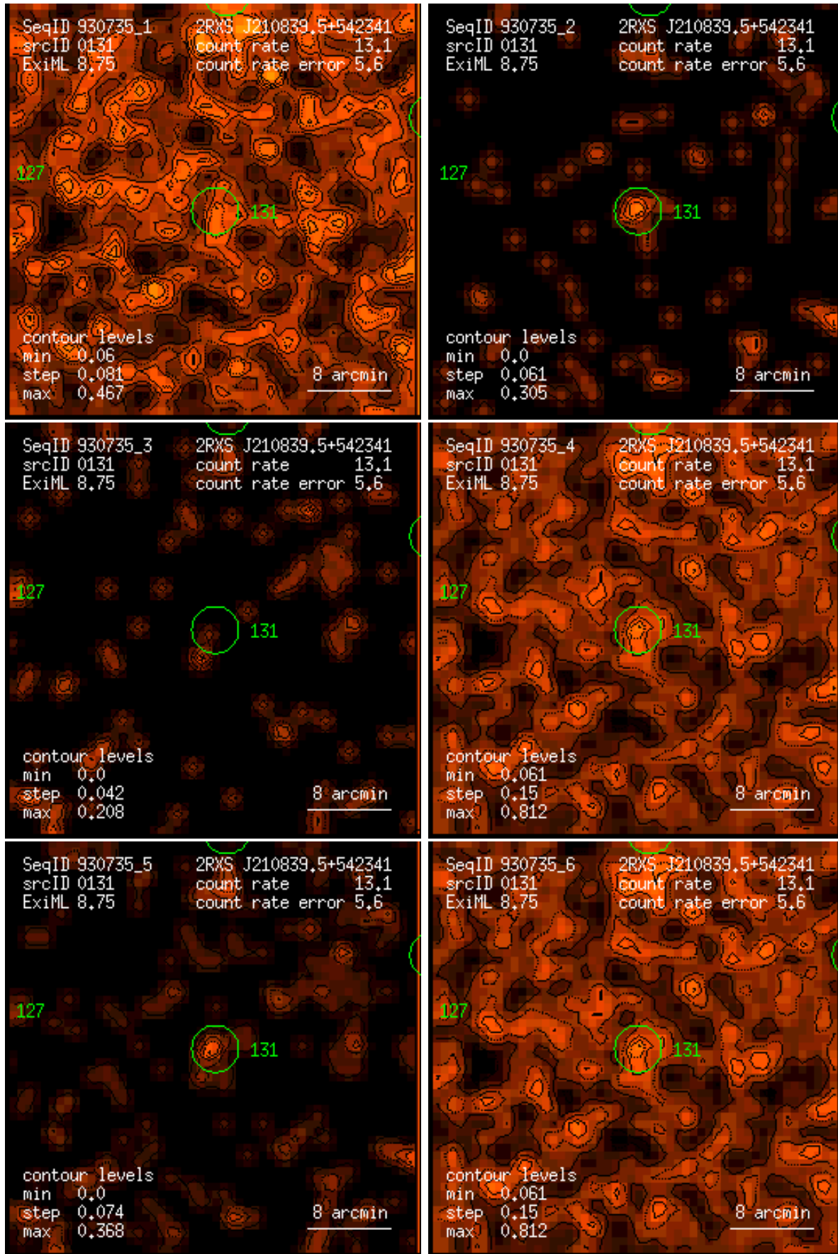
Figure 131: RASS 930735: detection 0131: band rate images, Gaussian filter: (1) PSPC channels 11 – 41, (2) 52 – 90, (3) 91 – 201, (4) 11 – 235, (5) 52 – 201, (6) 11 – 201. Broad band rates in counts/ks. Band rate contour levels in counts/ks/arcmin 2 .
