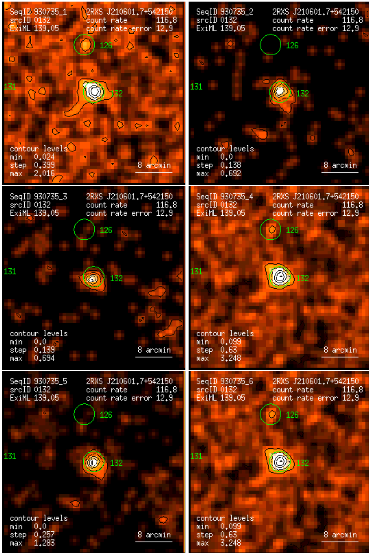
Figure 132: RASS 930735: detection 0132: band rate images, Gaussian filter: (1) PSPC channels 11 – 41, (2) 52 – 90, (3) 91 – 201, (4) 11 – 235, (5) 52 – 201, (6) 11 – 201. Broad band rates in counts/ks. Band rate contour levels in counts/ks/arcmin 2 .
