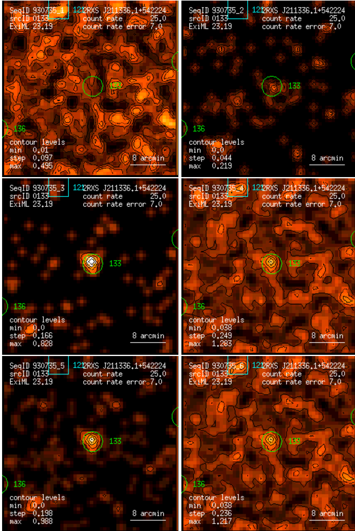
Figure 133: RASS 930735: detection 0133: band rate images, Gaussian filter: (1) PSPC channels 11 – 41, (2) 52 – 90, (3) 91 – 201, (4) 11 – 235, (5) 52 – 201, (6) 11 – 201. Broad band rates in counts/ks. Band rate contour levels in counts/ks/arcmin 2 .
