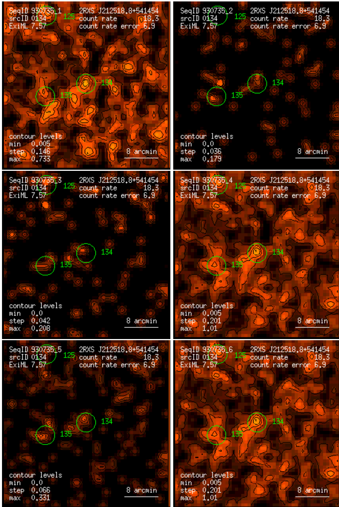
Figure 134: RASS 930735: detection 0134: band rate images, Gaussian filter: (1) PSPC channels 11 – 41, (2) 52 – 90, (3) 91 – 201, (4) 11 – 235, (5) 52 – 201, (6) 11 – 201. Broad band rates in counts/ks. Band rate contour levels in counts/ks/arcmin 2 .
