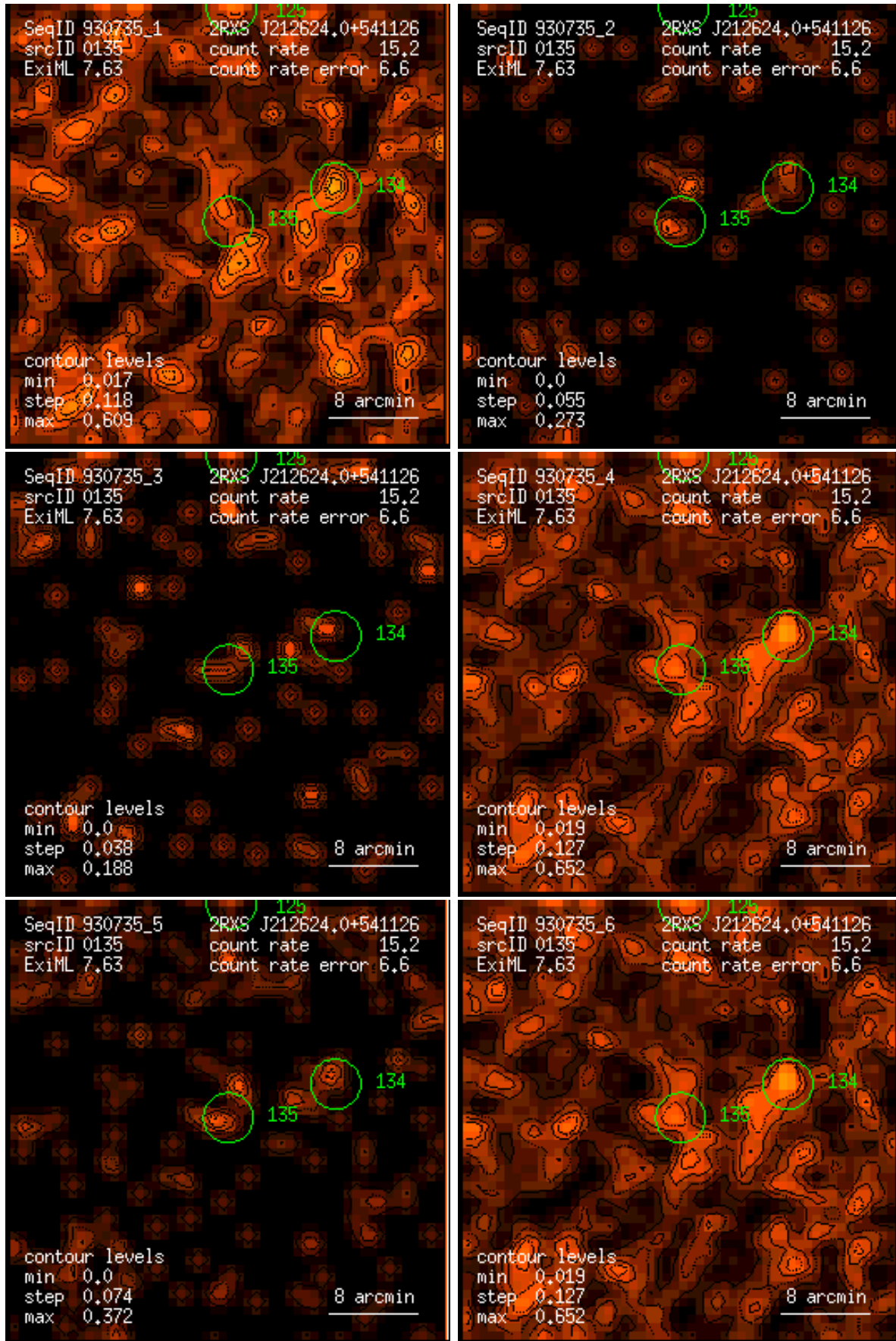
Figure 135: RASS 930735: detection 0135: band rate images, Gaussian filter: (1) PSPC channels 11 – 41, (2) 52 – 90, (3) 91 – 201, (4) 11 – 235, (5) 52 – 201, (6) 11 – 201. Broad band rates in counts/ks. Band rate contour levels in counts/ks/arcmin 2 .
