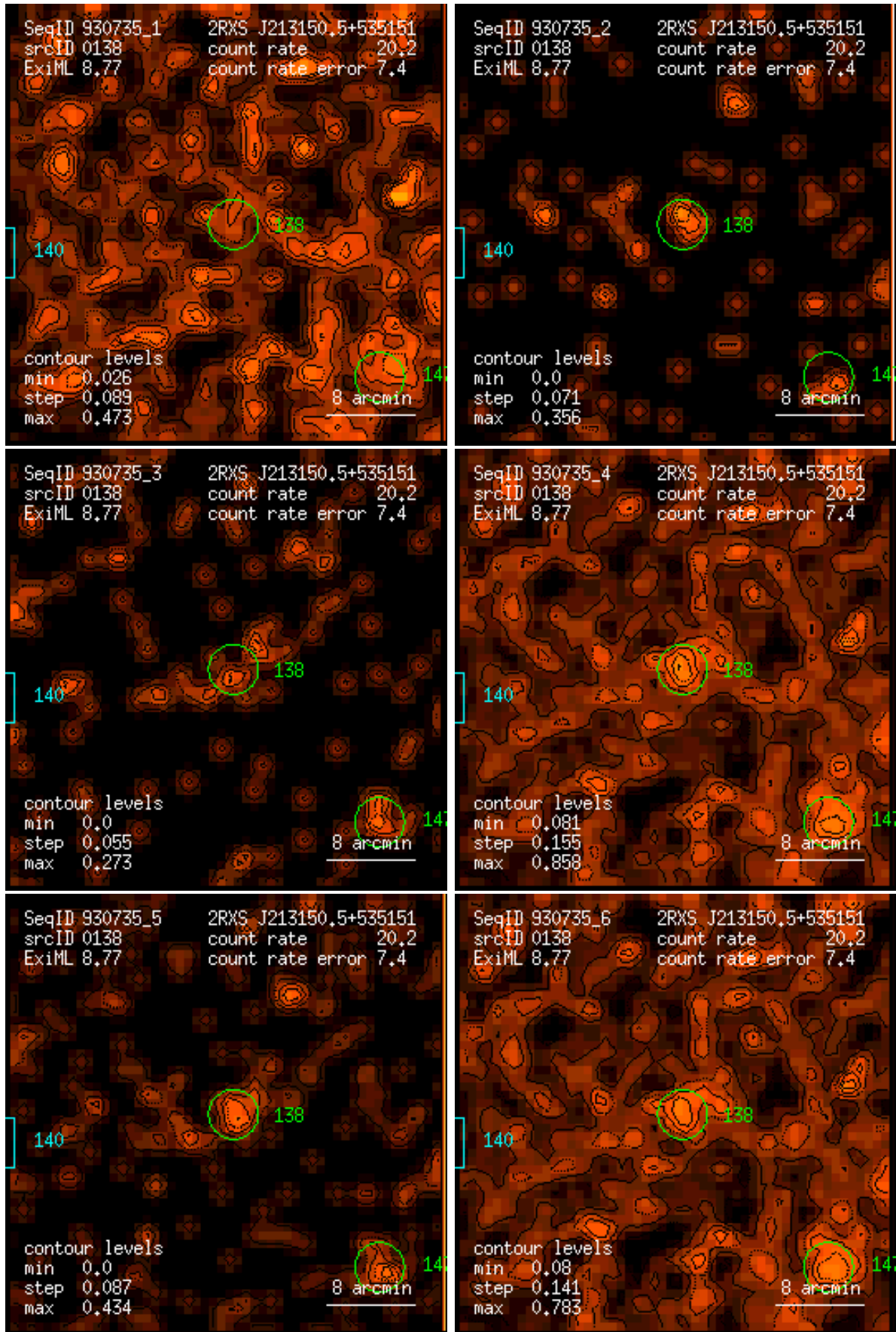
Figure 138: RASS 930735: detection 0138: band rate images, Gaussian filter: (1) PSPC channels 11 – 41, (2) 52 – 90, (3) 91 – 201, (4) 11 – 235, (5) 52 – 201, (6) 11 – 201. Broad band rates in counts/ks. Band rate contour levels in counts/ks/arcmin 2 .
