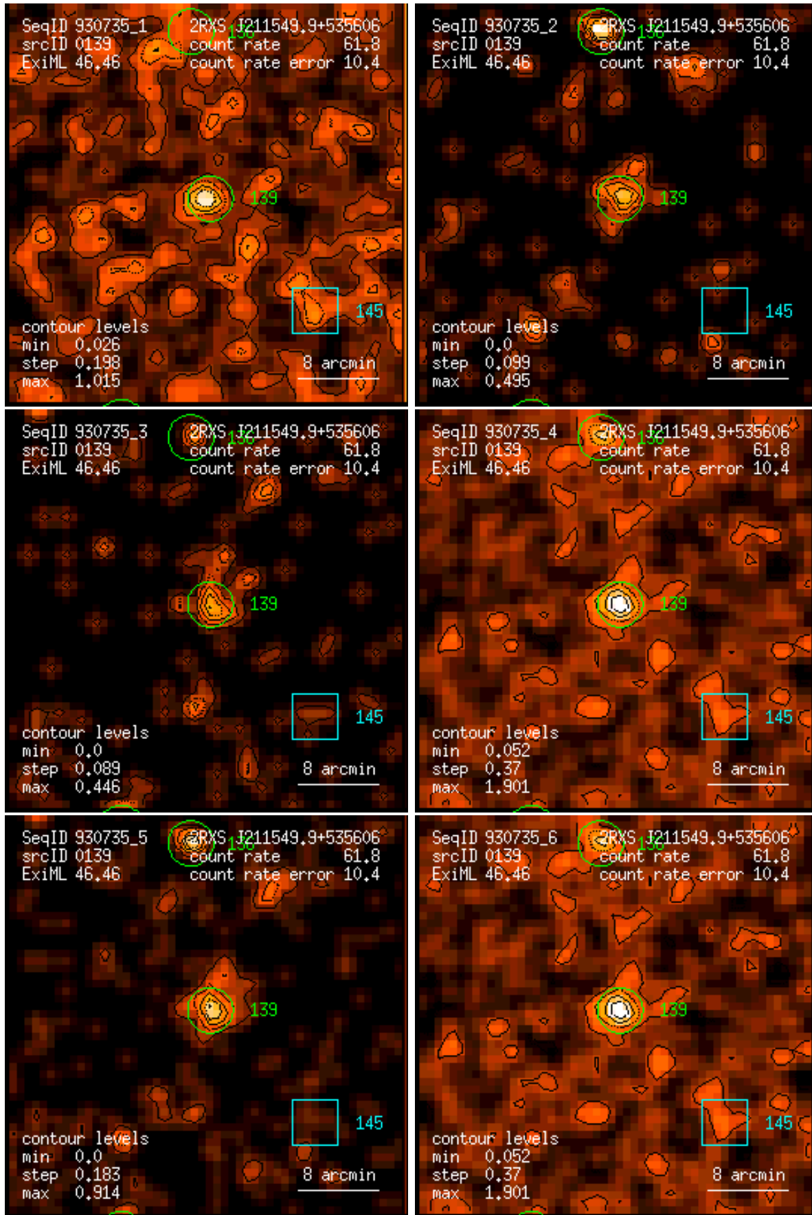
Figure 139: RASS 930735: detection 0139: band rate images, Gaussian filter: (1) PSPC channels 11 – 41, (2) 52 – 90, (3) 91 – 201, (4) 11 – 235, (5) 52 – 201, (6) 11 – 201. Broad band rates in counts/ks. Band rate contour levels in counts/ks/arcmin 2 .
