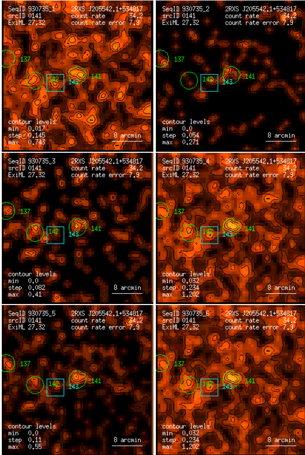
Figure 141: RASS 930735: detection 0141: band rate images, Gaussian filter: (1) PSPC channels 11 – 41, (2) 52 – 90, (3) 91 – 201, (4) 11 – 235, (5) 52 – 201, (6) 11 – 201. Broad band rates in counts/ks. Band rate contour levels in counts/ks/arcmin 2 .
