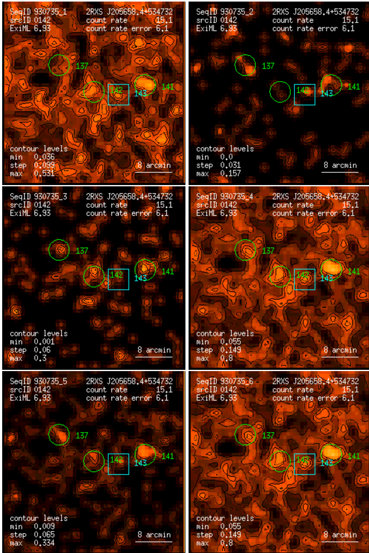
Figure 142: RASS 930735: detection 0142: band rate images, Gaussian filter: (1) PSPC channels 11 – 41, (2) 52 – 90, (3) 91 – 201, (4) 11 – 235, (5) 52 – 201, (6) 11 – 201. Broad band rates in counts/ks. Band rate contour levels in counts/ks/arcmin 2 .
