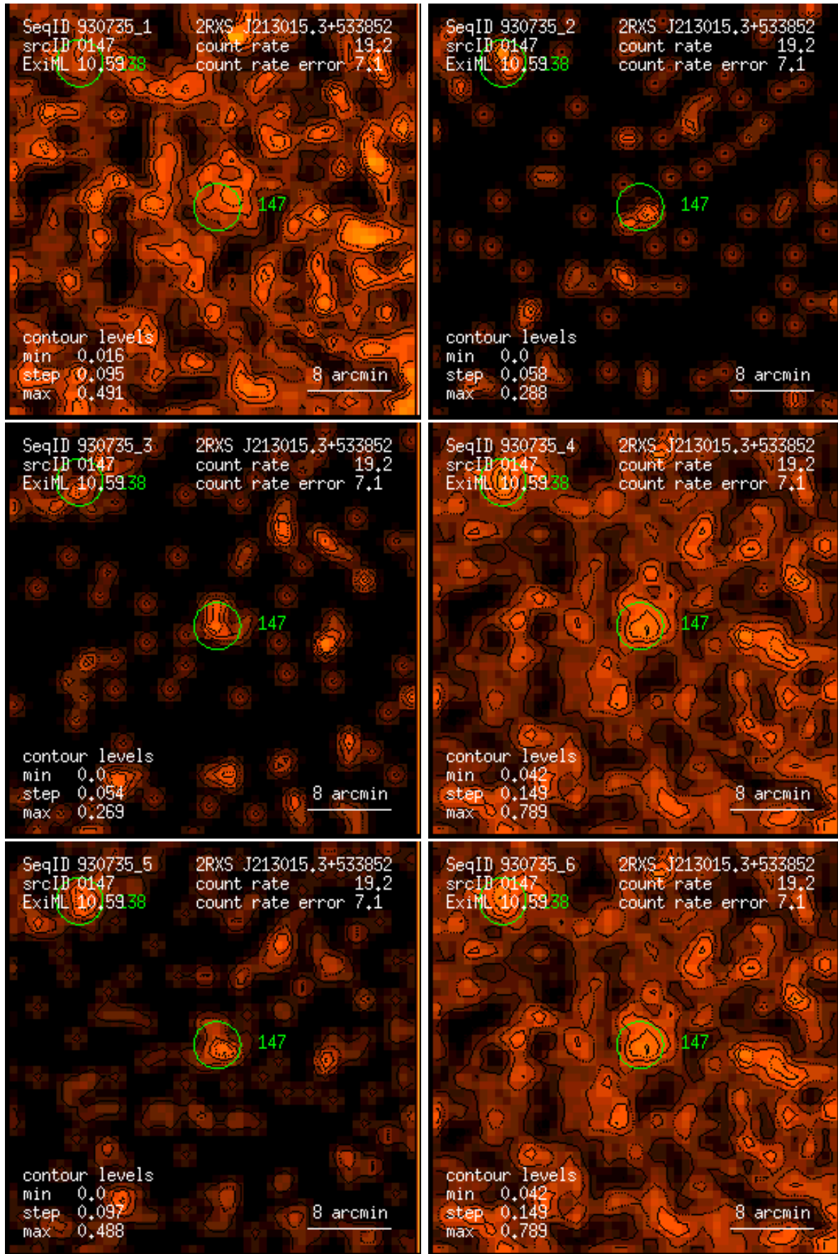
Figure 147: RASS 930735: detection 0147: band rate images, Gaussian filter: (1) PSPC channels 11 – 41, (2) 52 – 90, (3) 91 – 201, (4) 11 – 235, (5) 52 – 201, (6) 11 – 201. Broad band rates in counts/ks. Band rate contour levels in counts/ks/arcmin 2 .
