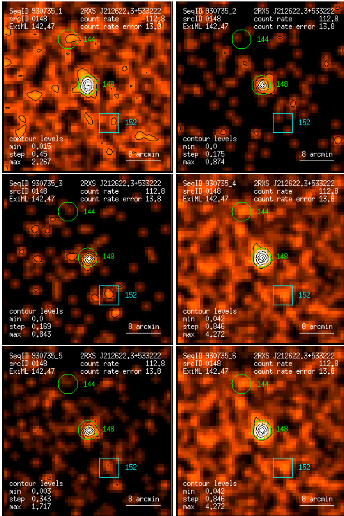
Figure 148: RASS 930735: detection 0148: band rate images, Gaussian filter: (1) PSPC channels 11 – 41, (2) 52 – 90, (3) 91 – 201, (4) 11 – 235, (5) 52 – 201, (6) 11 – 201. Broad band rates in counts/ks. Band rate contour levels in counts/ks/arcmin 2 .
