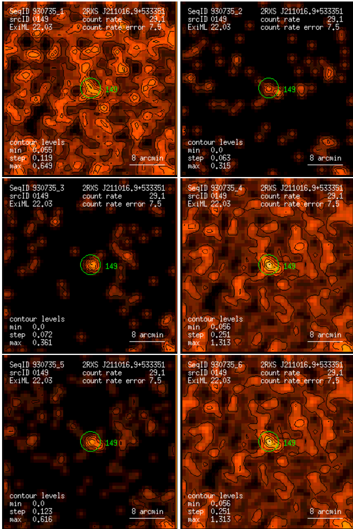
Figure 149: RASS 930735: detection 0149: band rate images, Gaussian filter: (1) PSPC channels 11 – 41, (2) 52 – 90, (3) 91 – 201, (4) 11 – 235, (5) 52 – 201, (6) 11 – 201. Broad band rates in counts/ks. Band rate contour levels in counts/ks/arcmin 2 .
