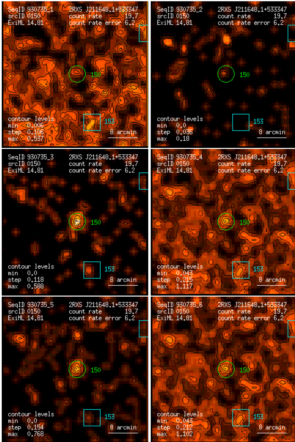
Figure 150: RASS 930735: detection 0150: band rate images, Gaussian filter: (1) PSPC channels 11 – 41, (2) 52 – 90, (3) 91 – 201, (4) 11 – 235, (5) 52 – 201, (6) 11 – 201. Broad band rates in counts/ks. Band rate contour levels in counts/ks/arcmin 2 .
