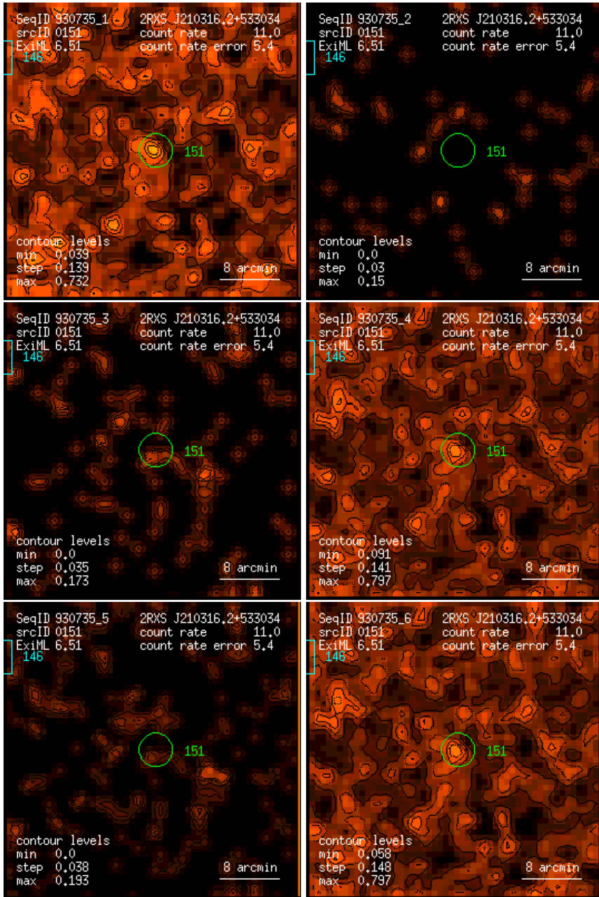
Figure 151: RASS 930735: detection 0151: band rate images, Gaussian filter: (1) PSPC channels 11 – 41, (2) 52 – 90, (3) 91 – 201, (4) 11 – 235, (5) 52 – 201, (6) 11 – 201. Broad band rates in counts/ks. Band rate contour levels in counts/ks/arcmin 2 .
