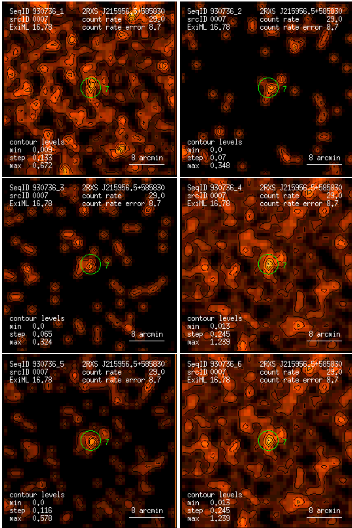
Figure 7: RASS 930736: detection 0007: band rate images, Gaussian filter: (1) PSPC channels 11 – 41, (2) 52 – 90, (3) 91 – 201, (4) 11 – 235, (5) 52 – 201, (6) 11 – 201. Broad band rates in counts/ks. Band rate contour levels in counts/ks/arcmin 2 .
