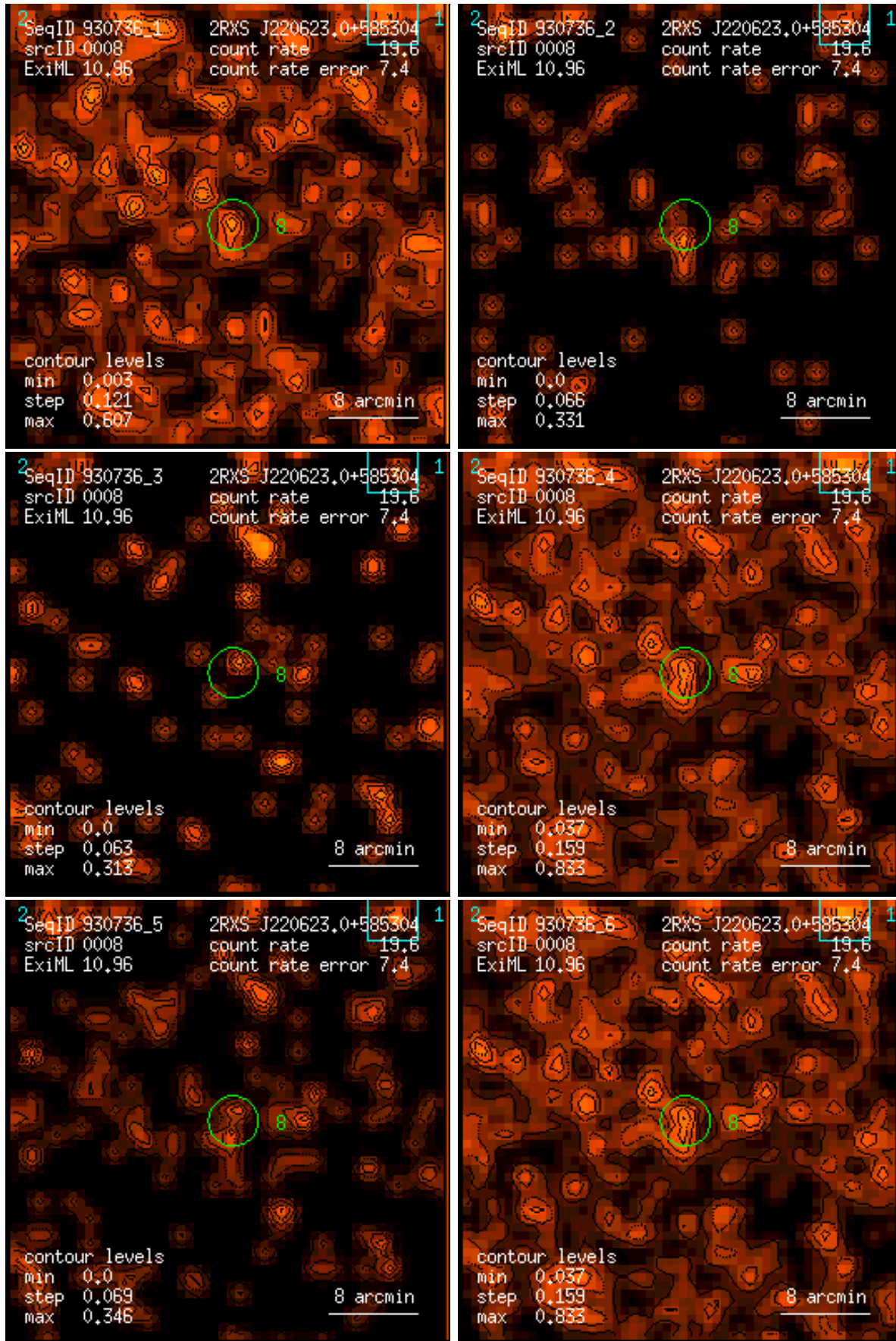
Figure 8: RASS 930736: detection 0008: band rate images, Gaussian filter: (1) PSPC channels 11 – 41, (2) 52 – 90, (3) 91 – 201, (4) 11 – 235, (5) 52 – 201, (6) 11 – 201. Broad band rates in counts/ks. Band rate contour levels in counts/ks/arcmin 2 .
