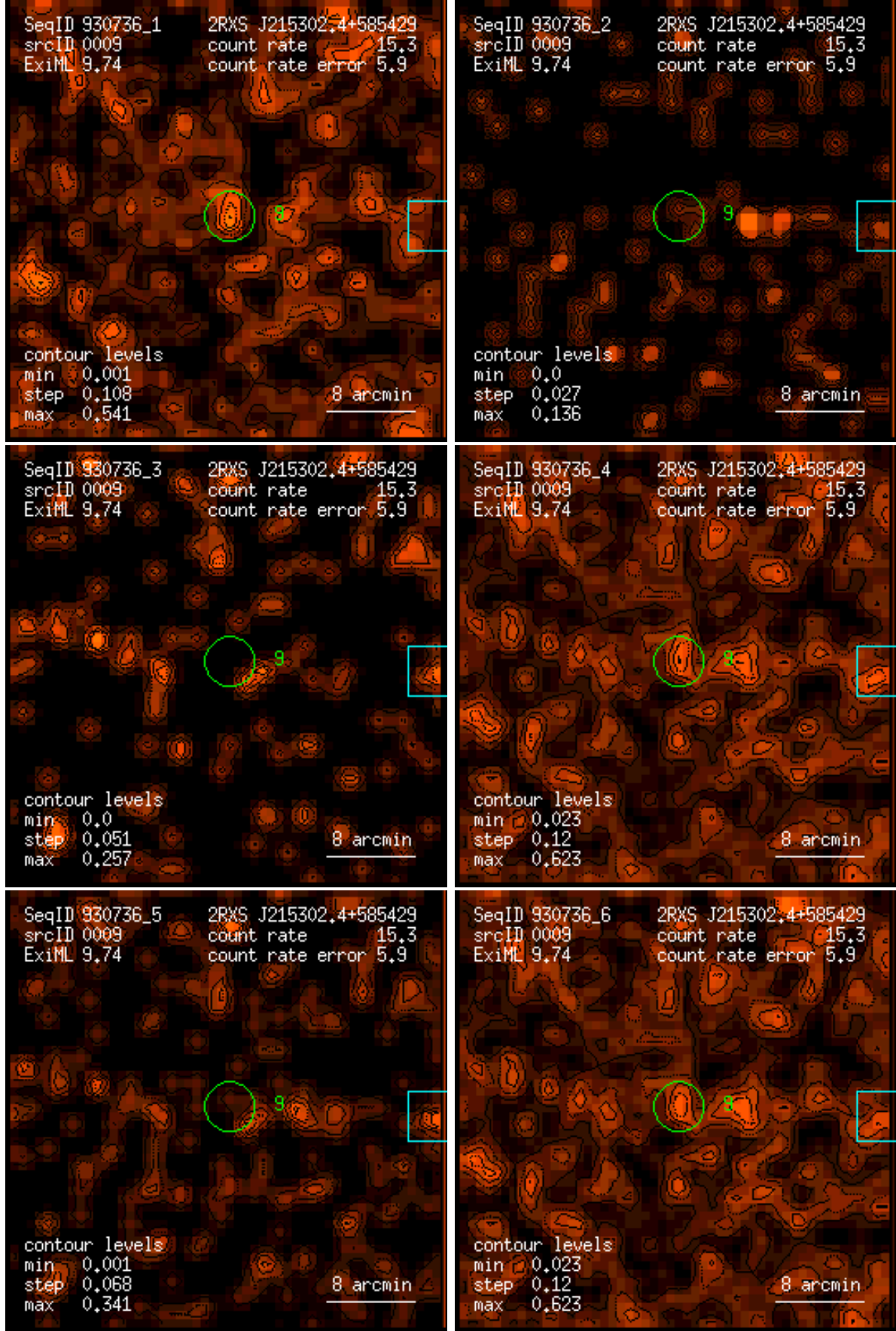
Figure 9: RASS 930736: detection 0009: band rate images, Gaussian filter: (1) PSPC channels 11 – 41, (2) 52 – 90, (3) 91 – 201, (4) 11 – 235, (5) 52 – 201, (6) 11 – 201. Broad band rates in counts/ks. Band rate contour levels in counts/ks/arcmin 2 .
