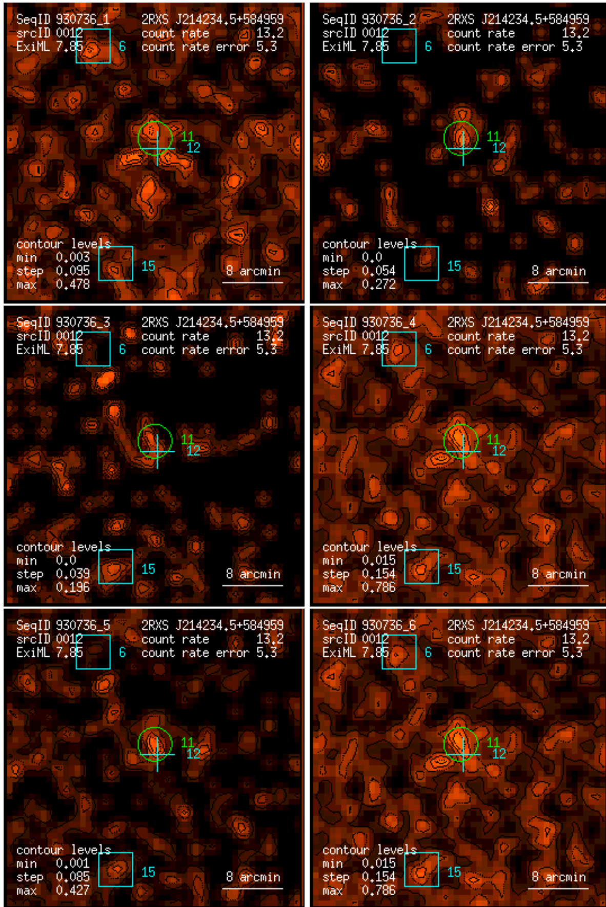
Figure 12: RASS 930736: detection 0012: band rate images, Gaussian filter: (1) PSPC channels 11 – 41, (2) 52 – 90, (3) 91 – 201, (4) 11 – 235, (5) 52 – 201, (6) 11 – 201. Broad band rates in counts/ks. Band rate contour levels in counts/ks/arcmin 2 .
