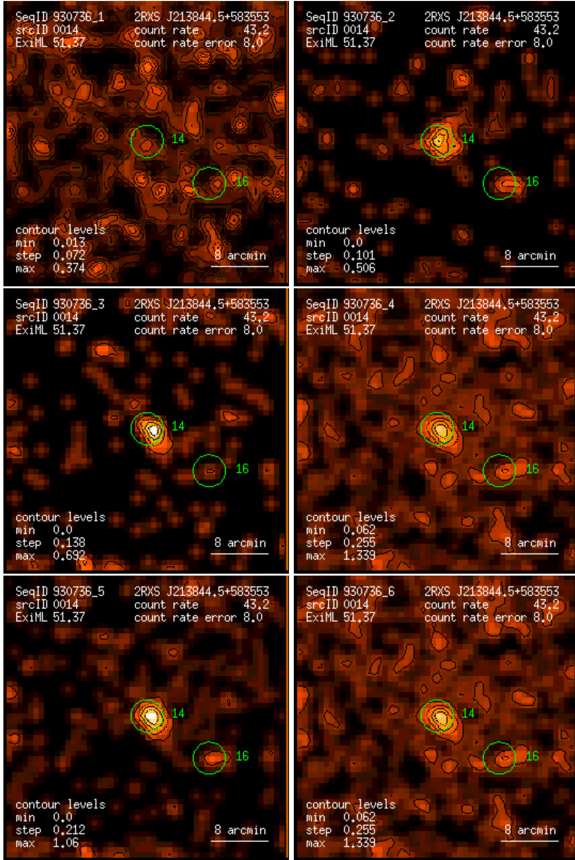
Figure 14: RASS 930736: detection 0014: band rate images, Gaussian filter: (1) PSPC channels 11 – 41, (2) 52 – 90, (3) 91 – 201, (4) 11 – 235, (5) 52 – 201, (6) 11 – 201. Broad band rates in counts/ks. Band rate contour levels in counts/ks/arcmin 2 .
