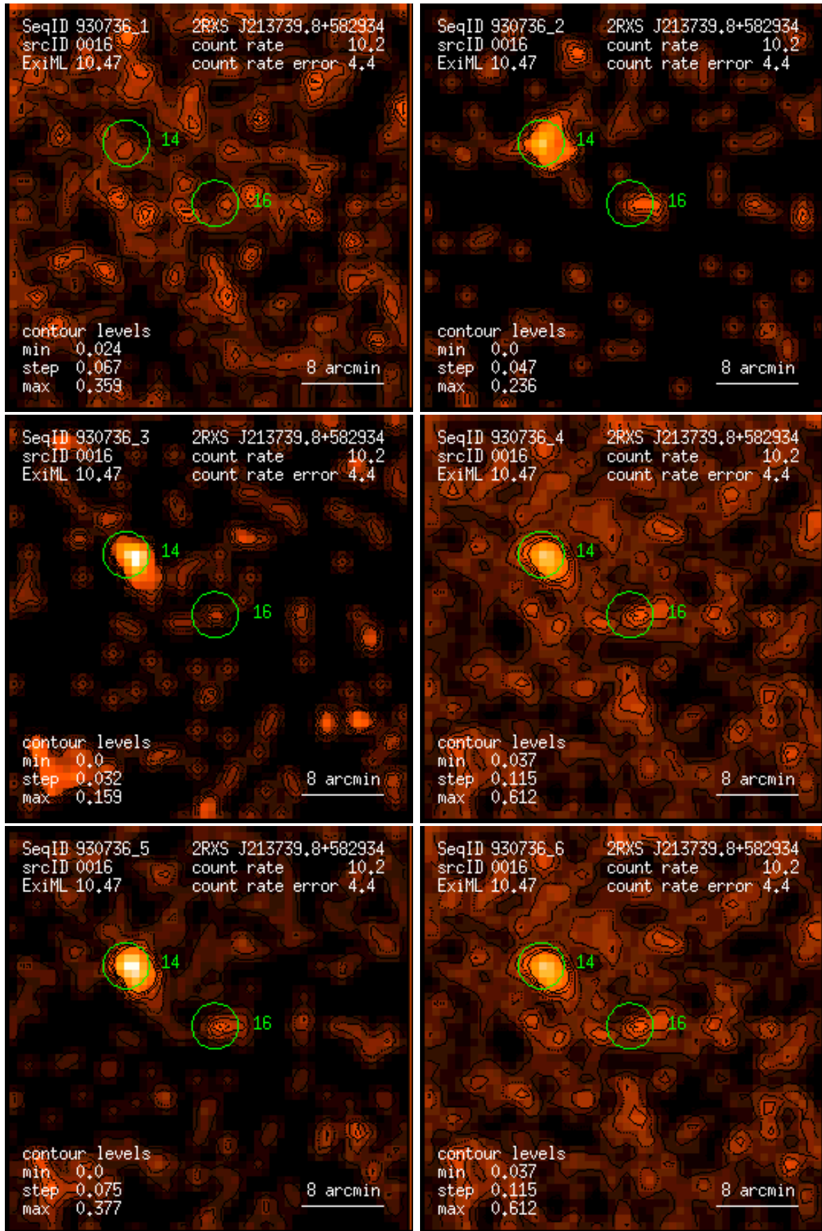
Figure 16: RASS 930736: detection 0016: band rate images, Gaussian filter: (1) PSPC channels 11 – 41, (2) 52 – 90, (3) 91 – 201, (4) 11 – 235, (5) 52 – 201, (6) 11 – 201. Broad band rates in counts/ks. Band rate contour levels in counts/ks/arcmin 2 .
