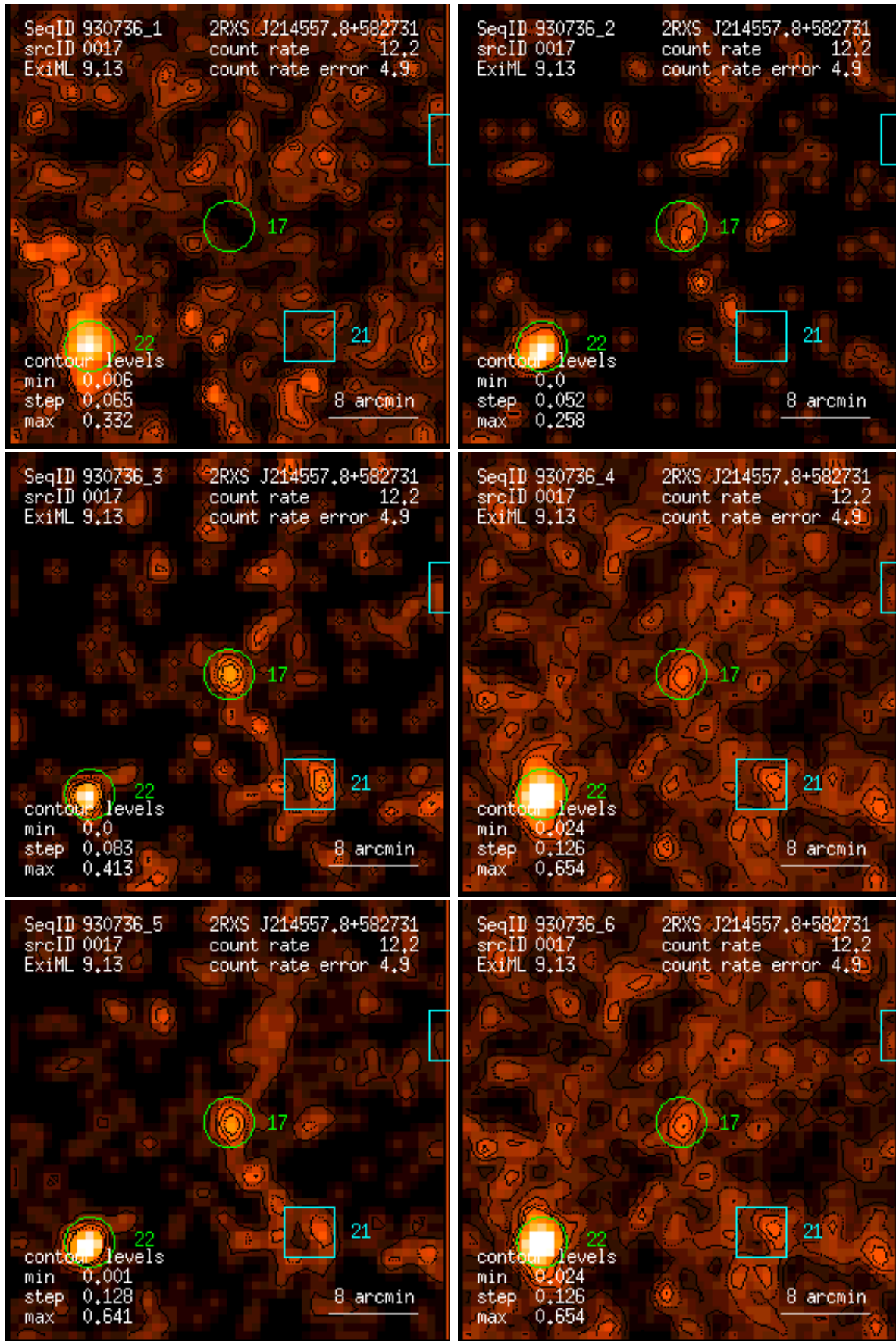
Figure 17: RASS 930736: detection 0017: band rate images, Gaussian filter: (1) PSPC channels 11 – 41, (2) 52 – 90, (3) 91 – 201, (4) 11 – 235, (5) 52 – 201, (6) 11 – 201. Broad band rates in counts/ks. Band rate contour levels in counts/ks/arcmin 2 .
