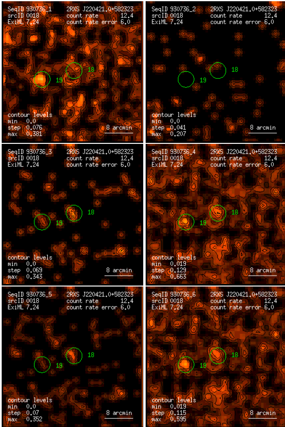
Figure 18: RASS 930736: detection 0018: band rate images, Gaussian filter: (1) PSPC channels 11 – 41, (2) 52 – 90, (3) 91 – 201, (4) 11 – 235, (5) 52 – 201, (6) 11 – 201. Broad band rates in counts/ks. Band rate contour levels in counts/ks/arcmin 2 .
