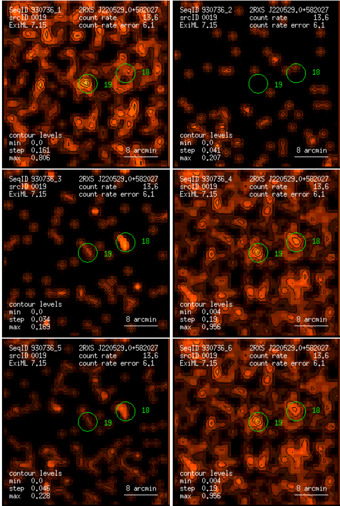
Figure 19: RASS 930736: detection 0019: band rate images, Gaussian filter: (1) PSPC channels 11 – 41, (2) 52 – 90, (3) 91 – 201, (4) 11 – 235, (5) 52 – 201, (6) 11 – 201. Broad band rates in counts/ks. Band rate contour levels in counts/ks/arcmin 2 .
