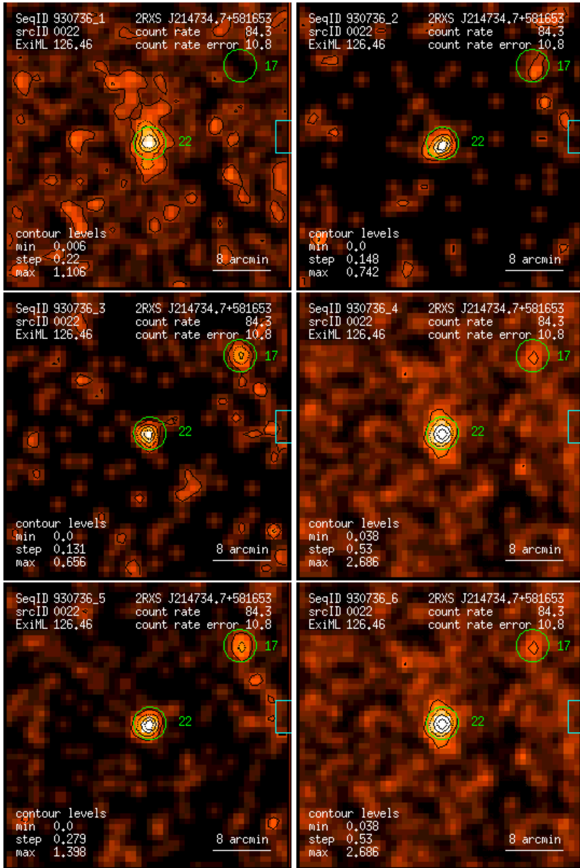
Figure 22: RASS 930736: detection 0022: band rate images, Gaussian filter: (1) PSPC channels 11 – 41, (2) 52 – 90, (3) 91 – 201, (4) 11 – 235, (5) 52 – 201, (6) 11 – 201. Broad band rates in counts/ks. Band rate contour levels in counts/ks/arcmin 2 .
